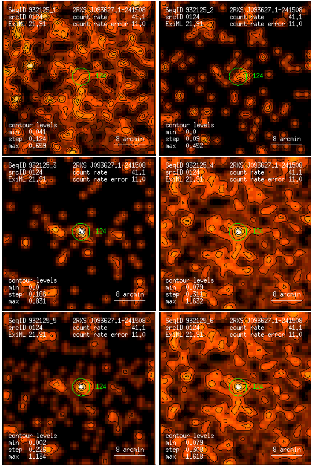
Figure 124: RASS 932125: detection 0124: band rate images, Gaussian filter: (1) PSPC channels 11 – 41, (2) 52 – 90, (3) 91 – 201, (4) 11 – 235, (5) 52 – 201, (6) 11 – 201. Broad band rates in counts/ks. Band rate contour levels in counts/ks/arcmin 2 .
