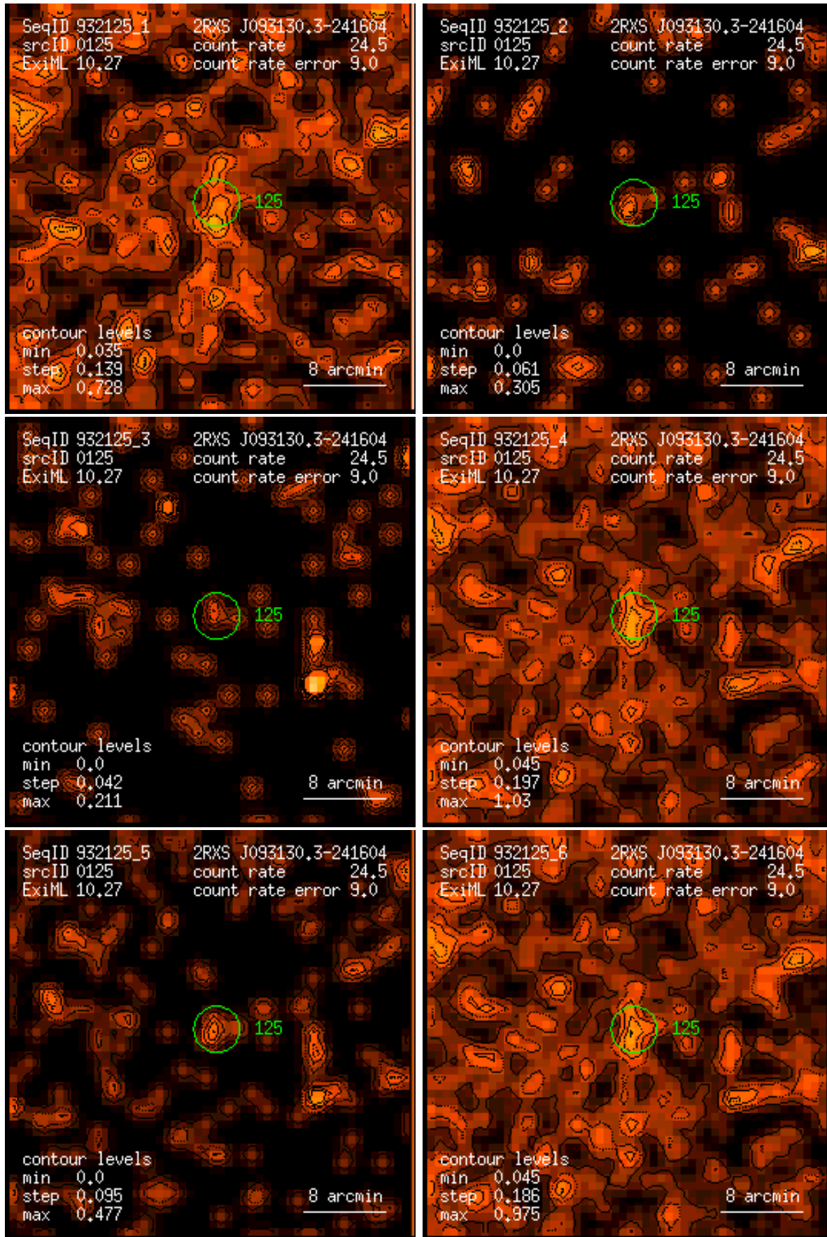
Figure 125: RASS 932125: detection 0125: band rate images, Gaussian filter: (1) PSPC channels 11 – 41, (2) 52 – 90, (3) 91 – 201, (4) 11 – 235, (5) 52 – 201, (6) 11 – 201. Broad band rates in counts/ks. Band rate contour levels in counts/ks/arcmin 2 .
