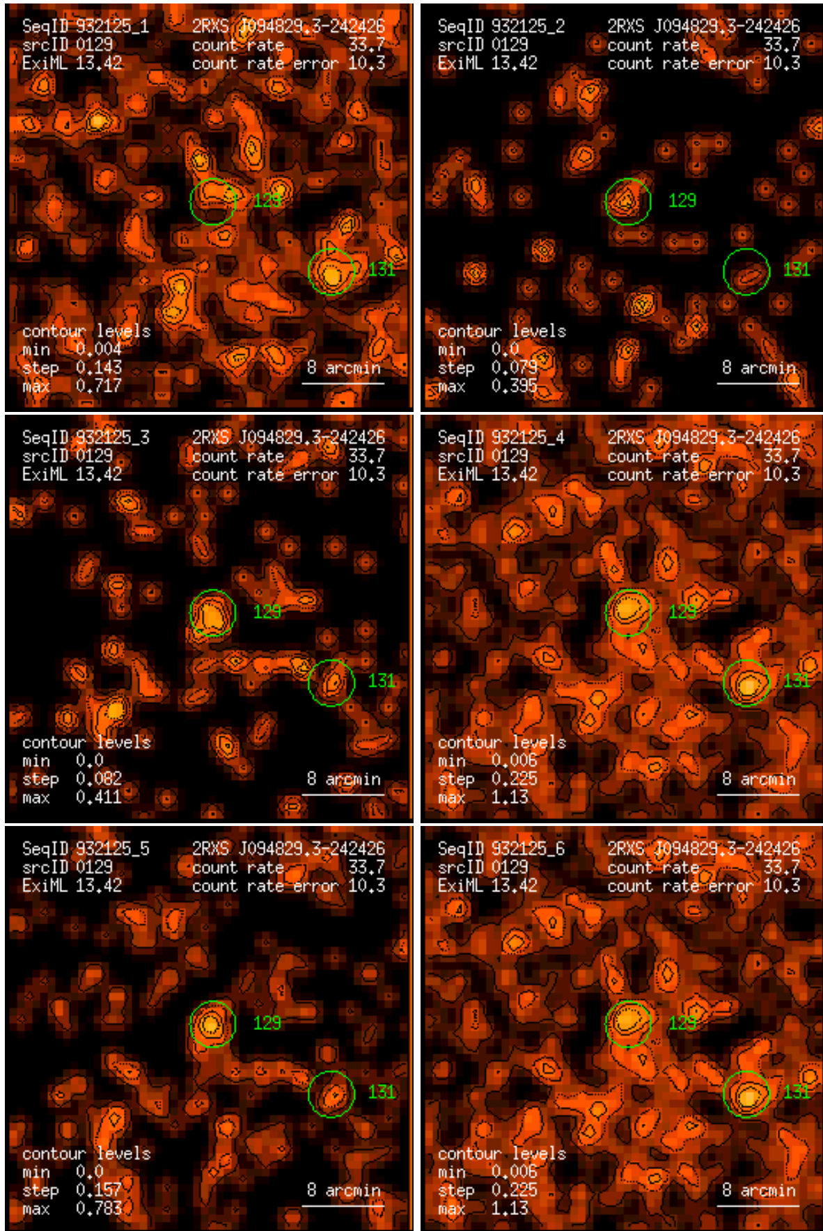
Figure 129: RASS 932125: detection 0129: band rate images, Gaussian filter: (1) PSPC channels 11 – 41, (2) 52 – 90, (3) 91 – 201, (4) 11 – 235, (5) 52 – 201, (6) 11 – 201. Broad band rates in counts/ks. Band rate contour levels in counts/ks/arcmin 2 .
