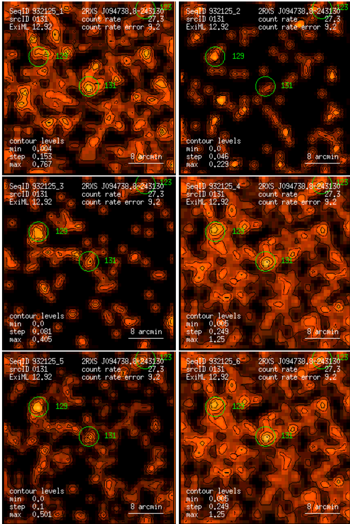
Figure 131: RASS 932125: detection 0131: band rate images, Gaussian filter: (1) PSPC channels 11 – 41, (2) 52 – 90, (3) 91 – 201, (4) 11 – 235, (5) 52 – 201, (6) 11 – 201. Broad band rates in counts/ks. Band rate contour levels in counts/ks/arcmin 2 .
