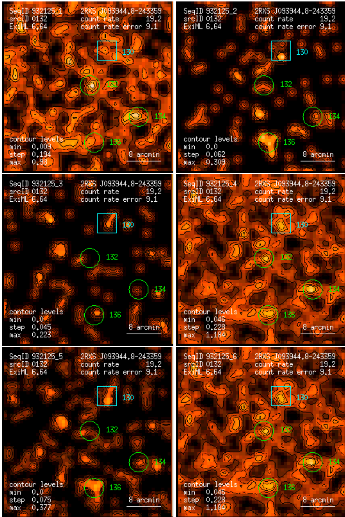
Figure 132: RASS 932125: detection 0132: band rate images, Gaussian filter: (1) PSPC channels 11 – 41, (2) 52 – 90, (3) 91 – 201, (4) 11 – 235, (5) 52 – 201, (6) 11 – 201. Broad band rates in counts/ks. Band rate contour levels in counts/ks/arcmin 2 .
