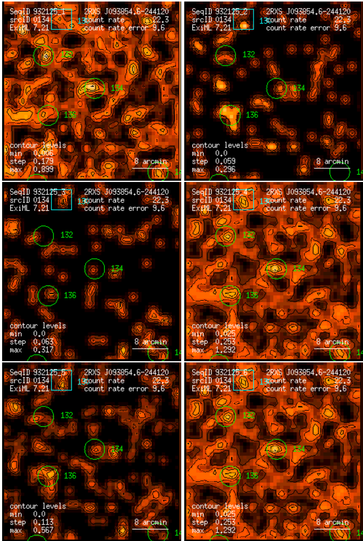
Figure 134: RASS 932125: detection 0134: band rate images, Gaussian filter: (1) PSPC channels 11 – 41, (2) 52 – 90, (3) 91 – 201, (4) 11 – 235, (5) 52 – 201, (6) 11 – 201. Broad band rates in counts/ks. Band rate contour levels in counts/ks/arcmin 2 .
