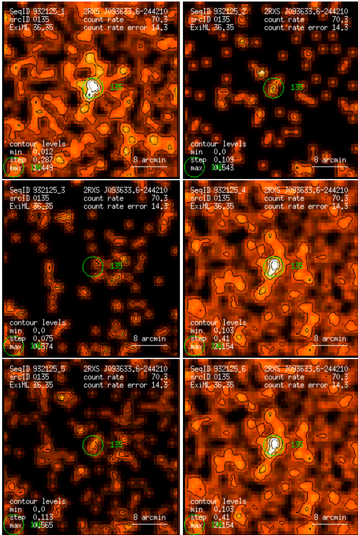
Figure 135: RASS 932125: detection 0135: band rate images, Gaussian filter: (1) PSPC channels 11 – 41, (2) 52 – 90, (3) 91 – 201, (4) 11 – 235, (5) 52 – 201, (6) 11 – 201. Broad band rates in counts/ks. Band rate contour levels in counts/ks/arcmin 2 .
