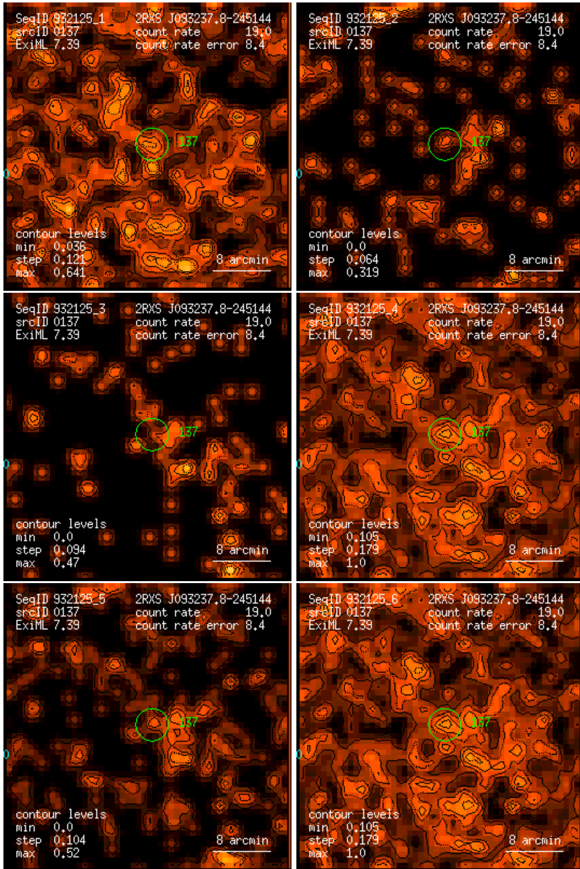
Figure 137: RASS 932125: detection 0137: band rate images, Gaussian filter: (1) PSPC channels 11 – 41, (2) 52 – 90, (3) 91 – 201, (4) 11 – 235, (5) 52 – 201, (6) 11 – 201. Broad band rates in counts/ks. Band rate contour levels in counts/ks/arcmin 2 .
