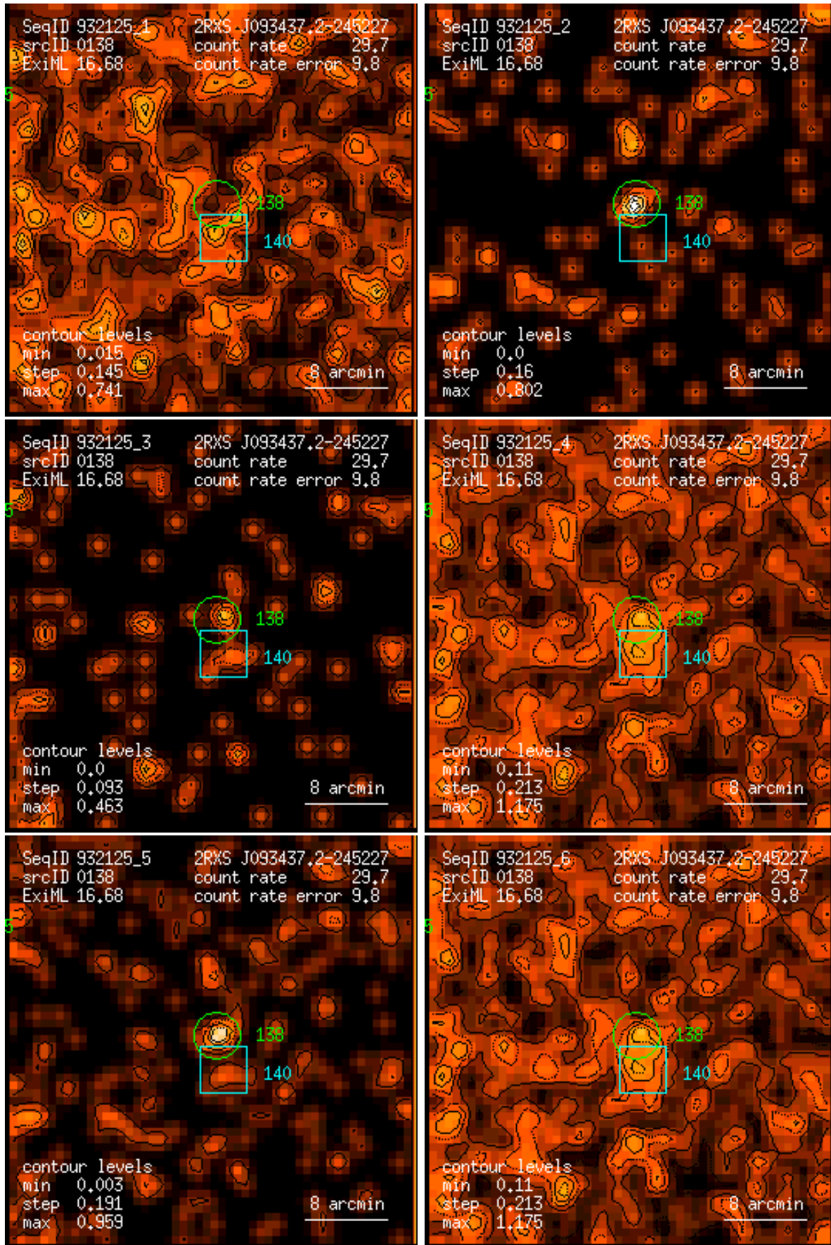
Figure 138: RASS 932125: detection 0138: band rate images, Gaussian filter: (1) PSPC channels 11 – 41, (2) 52 – 90, (3) 91 – 201, (4) 11 – 235, (5) 52 – 201, (6) 11 – 201. Broad band rates in counts/ks. Band rate contour levels in counts/ks/arcmin 2 .
