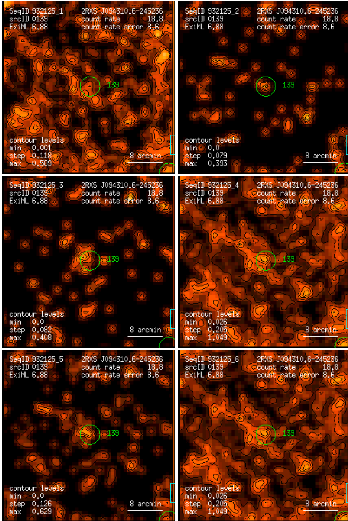
Figure 139: RASS 932125: detection 0139: band rate images, Gaussian filter: (1) PSPC channels 11 – 41, (2) 52 – 90, (3) 91 – 201, (4) 11 – 235, (5) 52 – 201, (6) 11 – 201. Broad band rates in counts/ks. Band rate contour levels in counts/ks/arcmin 2 .
