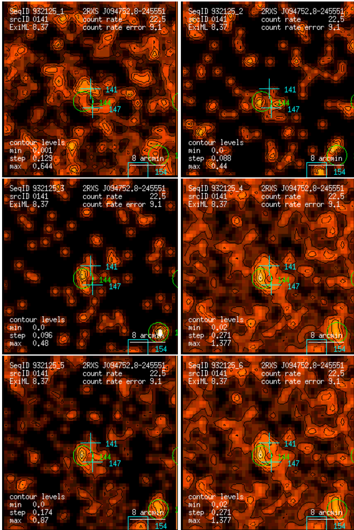
Figure 141: RASS 932125: detection 0141: band rate images, Gaussian filter: (1) PSPC channels 11 – 41, (2) 52 – 90, (3) 91 – 201, (4) 11 – 235, (5) 52 – 201, (6) 11 – 201. Broad band rates in counts/ks. Band rate contour levels in counts/ks/arcmin 2 .
