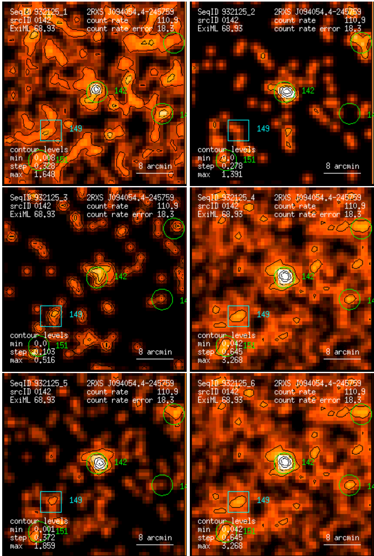
Figure 142: RASS 932125: detection 0142: band rate images, Gaussian filter: (1) PSPC channels 11 – 41, (2) 52 – 90, (3) 91 – 201, (4) 11 – 235, (5) 52 – 201, (6) 11 – 201. Broad band rates in counts/ks. Band rate contour levels in counts/ks/arcmin 2 .
