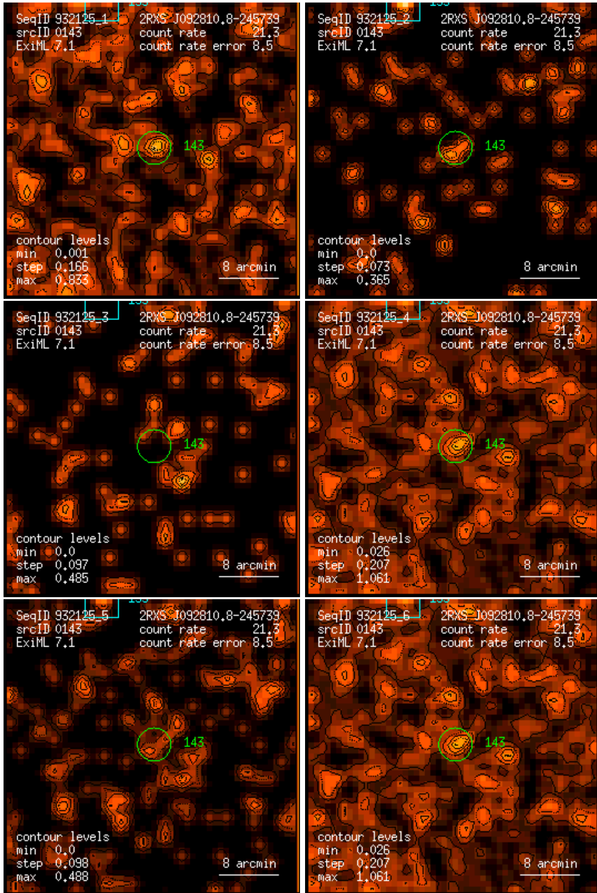
Figure 143: RASS 932125: detection 0143: band rate images, Gaussian filter: (1) PSPC channels 11 – 41, (2) 52 – 90, (3) 91 – 201, (4) 11 – 235, (5) 52 – 201, (6) 11 – 201. Broad band rates in counts/ks. Band rate contour levels in counts/ks/arcmin 2 .
