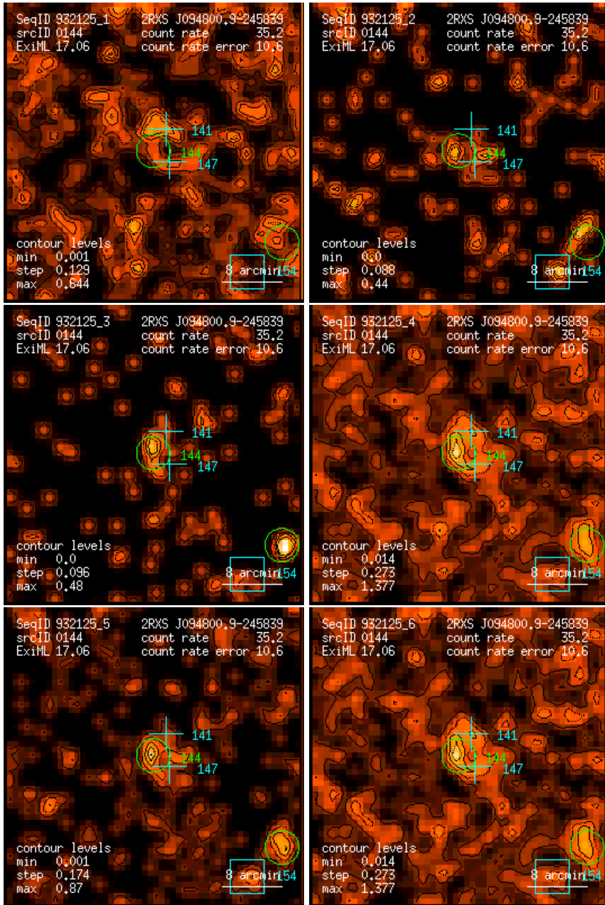
Figure 144: RASS 932125: detection 0144: band rate images, Gaussian filter: (1) PSPC channels 11 – 41, (2) 52 – 90, (3) 91 – 201, (4) 11 – 235, (5) 52 – 201, (6) 11 – 201. Broad band rates in counts/ks. Band rate contour levels in counts/ks/arcmin 2 .
