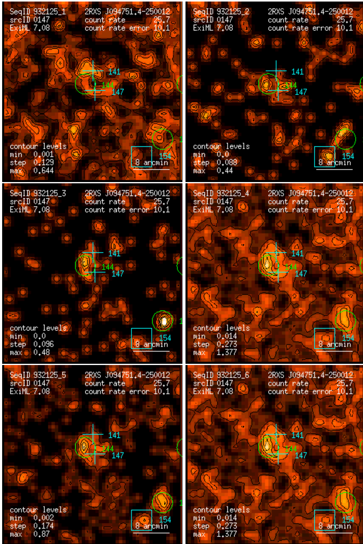
Figure 147: RASS 932125: detection 0147: band rate images, Gaussian filter: (1) PSPC channels 11 – 41, (2) 52 – 90, (3) 91 – 201, (4) 11 – 235, (5) 52 – 201, (6) 11 – 201. Broad band rates in counts/ks. Band rate contour levels in counts/ks/arcmin 2 .
