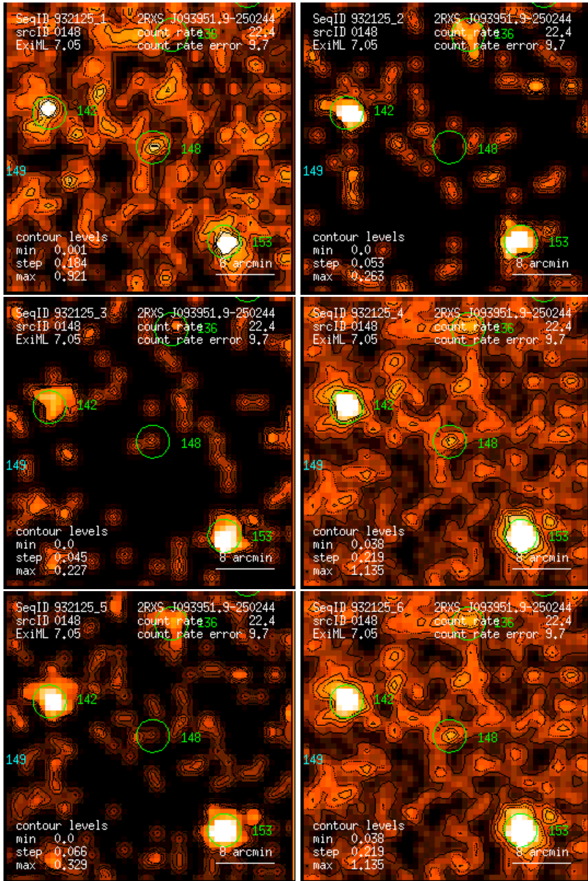
Figure 148: RASS 932125: detection 0148: band rate images, Gaussian filter: (1) PSPC channels 11 – 41, (2) 52 – 90, (3) 91 – 201, (4) 11 – 235, (5) 52 – 201, (6) 11 – 201. Broad band rates in counts/ks. Band rate contour levels in counts/ks/arcmin 2 .
