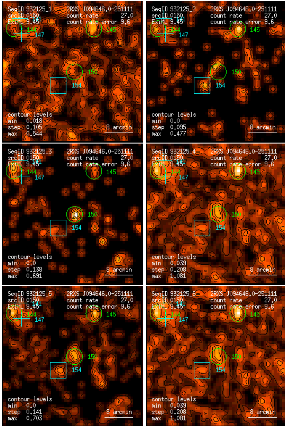
Figure 150: RASS 932125: detection 0150: band rate images, Gaussian filter: (1) PSPC channels 11 – 41, (2) 52 – 90, (3) 91 – 201, (4) 11 – 235, (5) 52 – 201, (6) 11 – 201. Broad band rates in counts/ks. Band rate contour levels in counts/ks/arcmin 2 .
