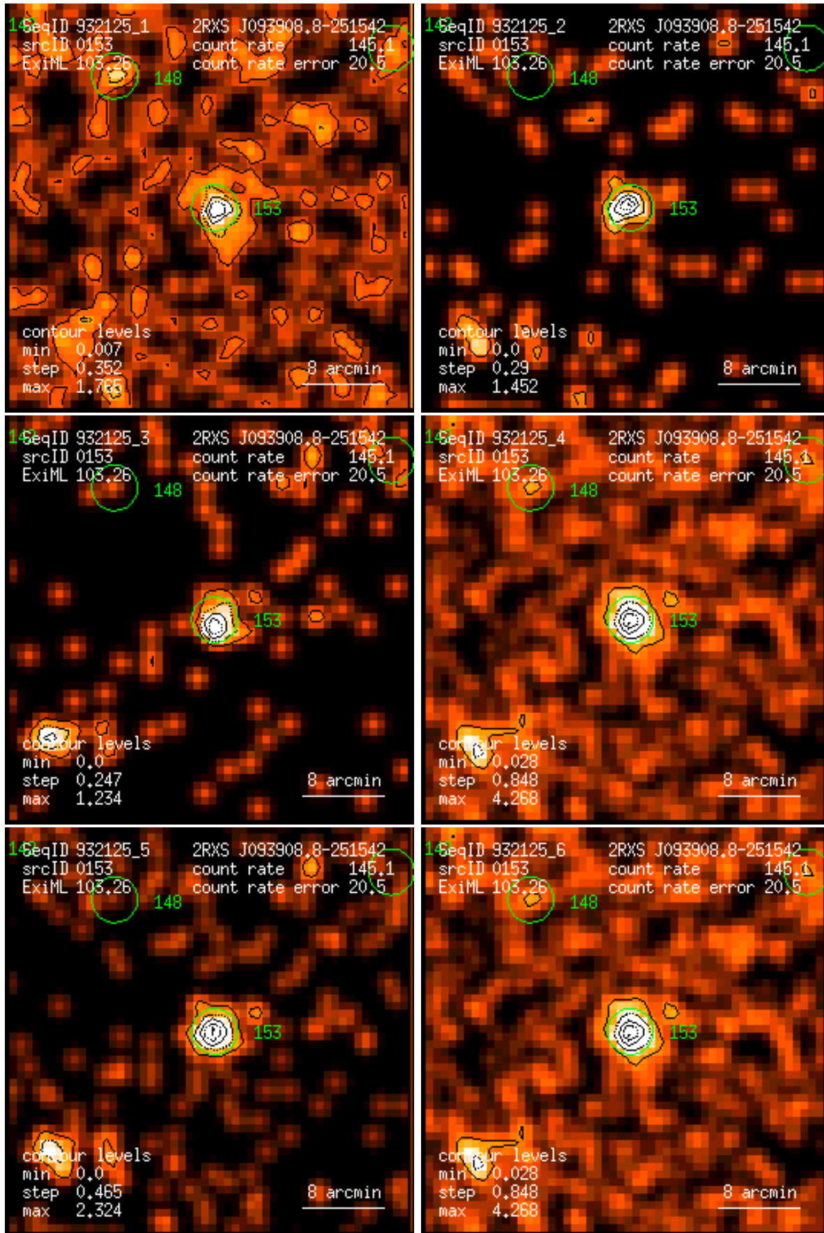
Figure 153: RASS 932125: detection 0153: band rate images, Gaussian filter: (1) PSPC channels 11 – 41, (2) 52 – 90, (3) 91 – 201, (4) 11 – 235, (5) 52 – 201, (6) 11 – 201. Broad band rates in counts/ks. Band rate contour levels in counts/ks/arcmin 2 .
