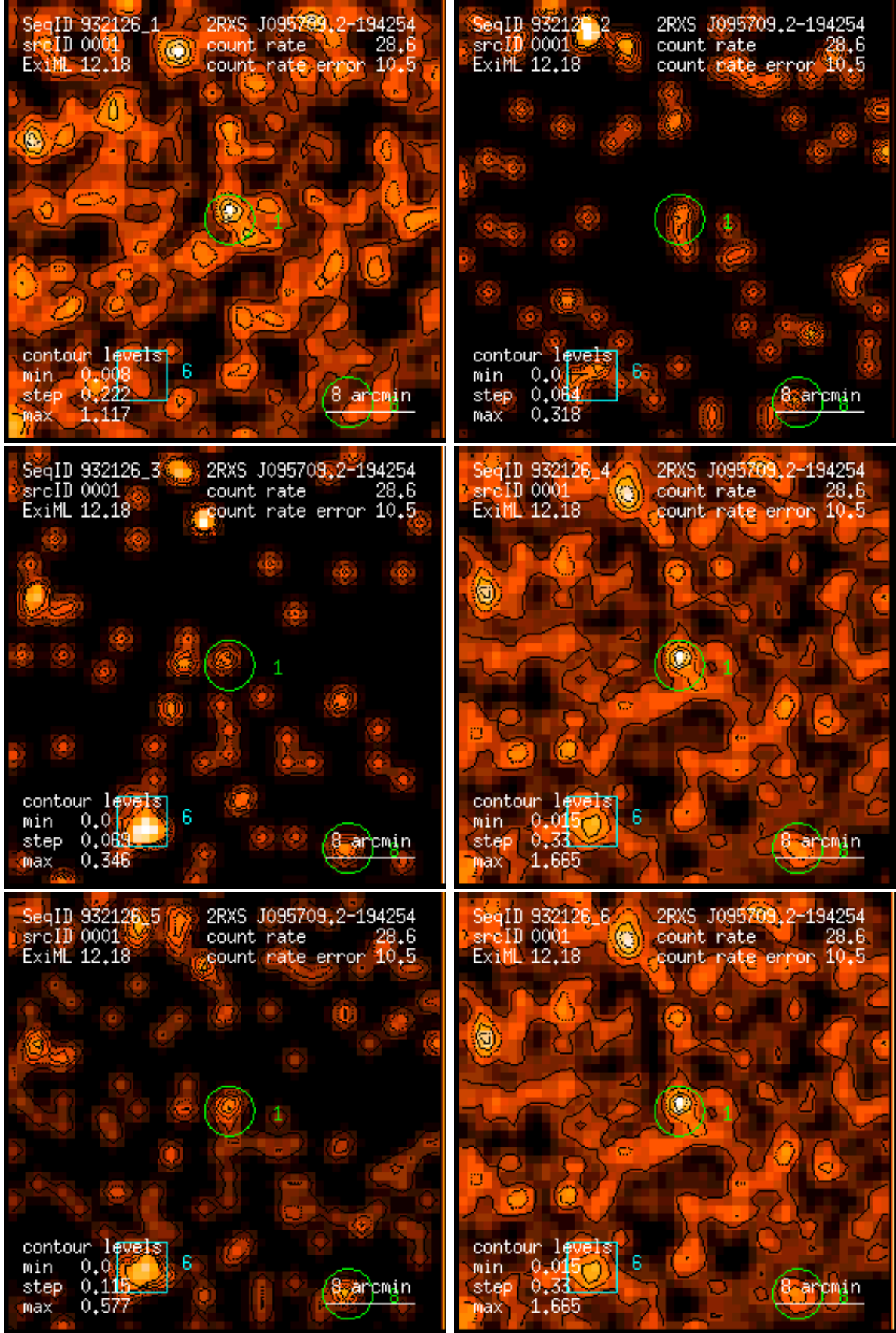
Figure 1: RASS 932126: detection 0001: band rate images, Gaussian filter: (1) PSPC channels 11 – 41, (2) 52 – 90, (3) 91 – 201, (4) 11 – 235, (5) 52 – 201, (6) 11 – 201. Broad band rates in counts/ks. Band rate contour levels in counts/ks/arcmin 2 .
