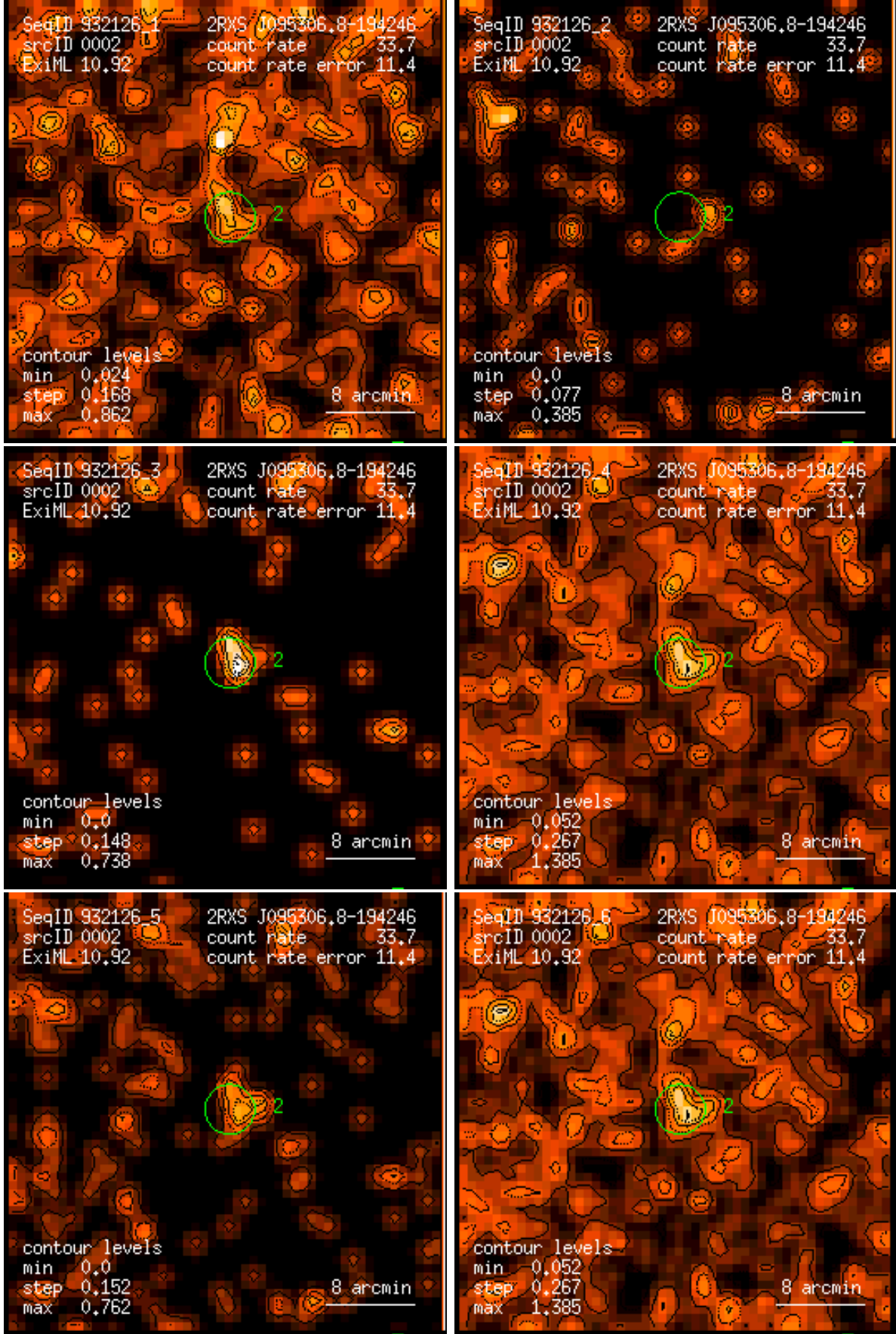
Figure 2: RASS 932126: detection 0002: band rate images, Gaussian filter: (1) PSPC channels 11 – 41, (2) 52 – 90, (3) 91 – 201, (4) 11 – 235, (5) 52 – 201, (6) 11 – 201. Broad band rates in counts/ks. Band rate contour levels in counts/ks/arcmin 2 .
