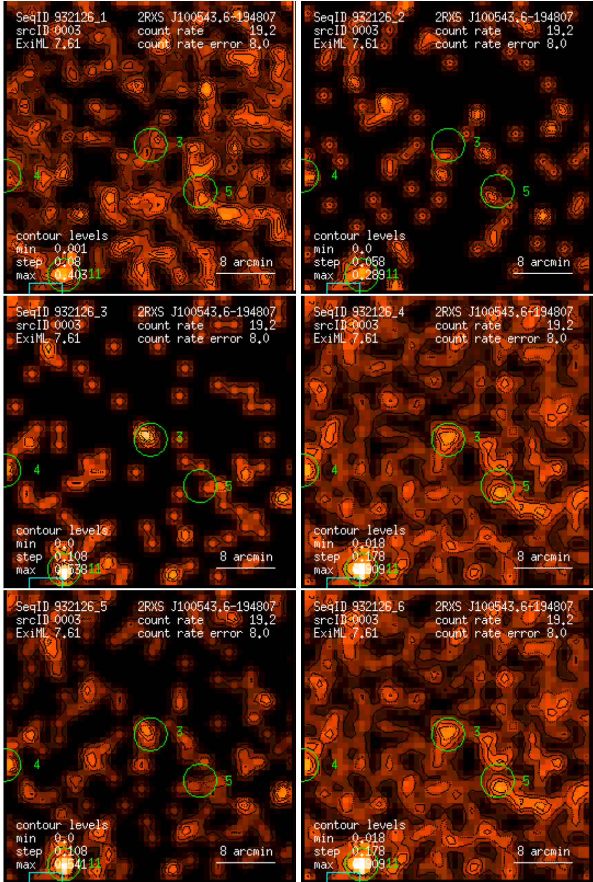
Figure 3: RASS 932126: detection 0003: band rate images, Gaussian filter: (1) PSPC channels 11 – 41, (2) 52 – 90, (3) 91 – 201, (4) 11 – 235, (5) 52 – 201, (6) 11 – 201. Broad band rates in counts/ks. Band rate contour levels in counts/ks/arcmin 2 .
