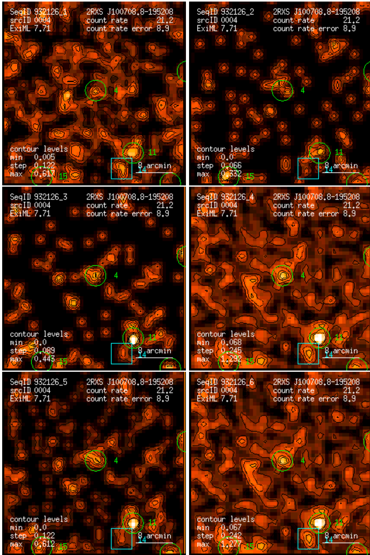
Figure 4: RASS 932126: detection 0004: band rate images, Gaussian filter: (1) PSPC channels 11 – 41, (2) 52 – 90, (3) 91 – 201, (4) 11 – 235, (5) 52 – 201, (6) 11 – 201. Broad band rates in counts/ks. Band rate contour levels in counts/ks/arcmin 2 .
