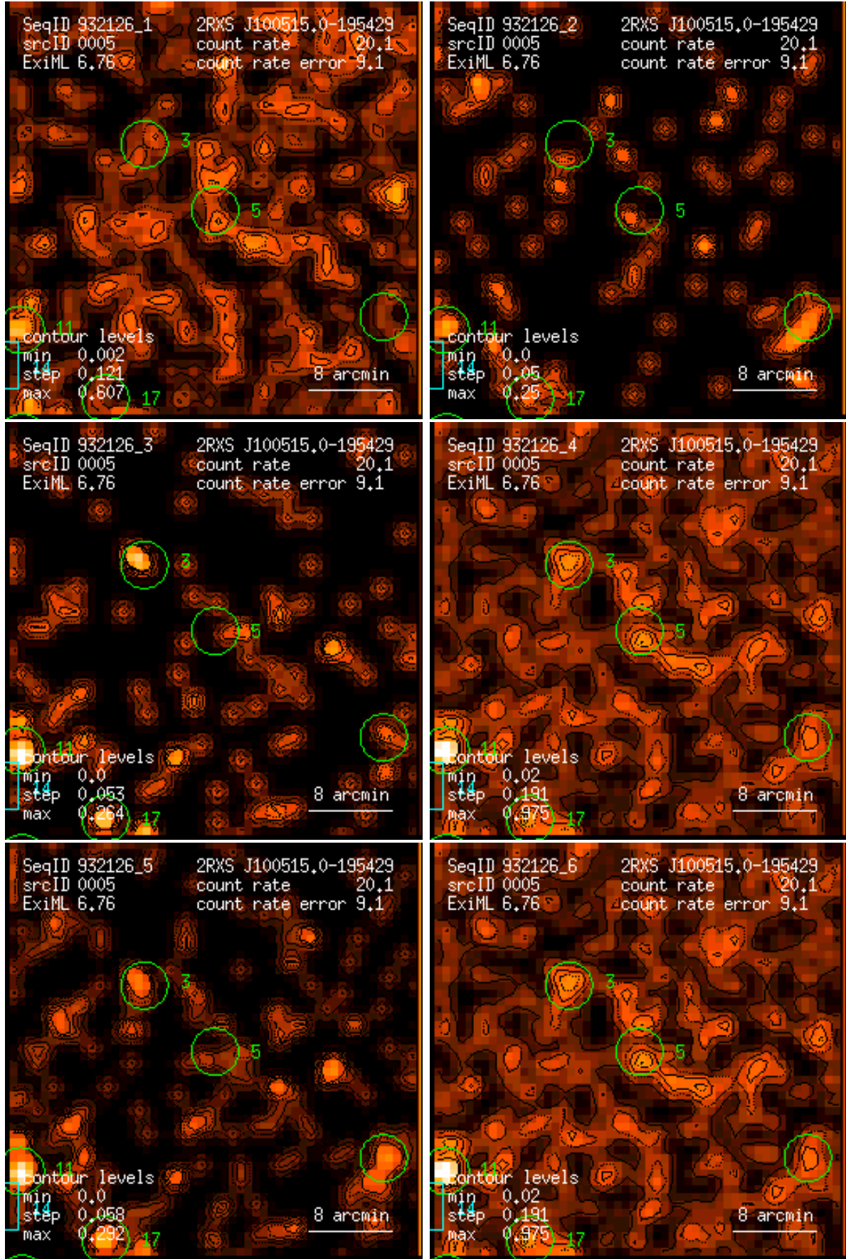
Figure 5: RASS 932126: detection 0005: band rate images, Gaussian filter: (1) PSPC channels 11 – 41, (2) 52 – 90, (3) 91 – 201, (4) 11 – 235, (5) 52 – 201, (6) 11 – 201. Broad band rates in counts/ks. Band rate contour levels in counts/ks/arcmin 2 .
