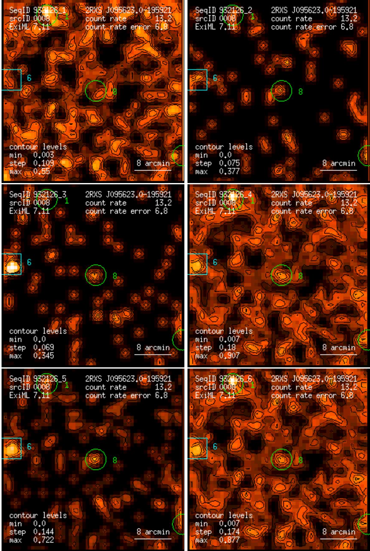
Figure 8: RASS 932126: detection 0008: band rate images, Gaussian filter: (1) PSPC channels 11 – 41, (2) 52 – 90, (3) 91 – 201, (4) 11 – 235, (5) 52 – 201, (6) 11 – 201. Broad band rates in counts/ks. Band rate contour levels in counts/ks/arcmin 2 .
