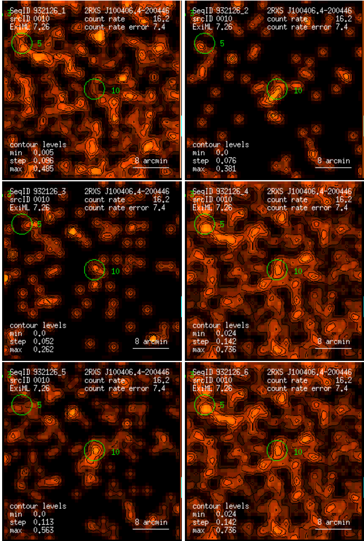
Figure 10: RASS 932126: detection 0010: band rate images, Gaussian filter: (1) PSPC channels 11 – 41, (2) 52 – 90, (3) 91 – 201, (4) 11 – 235, (5) 52 – 201, (6) 11 – 201. Broad band rates in counts/ks. Band rate contour levels in counts/ks/arcmin 2 .
