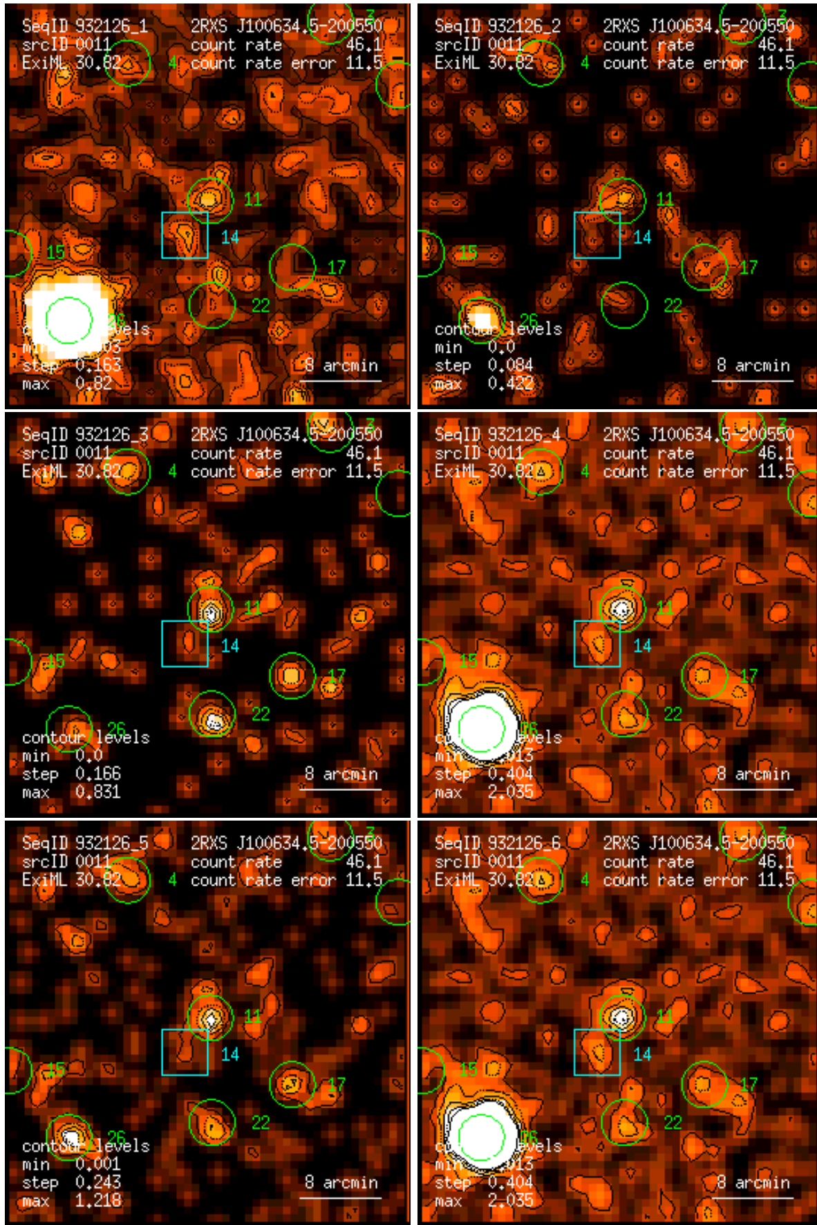
Figure 11: RASS 932126: detection 0011: band rate images, Gaussian filter: (1) PSPC channels 11 – 41, (2) 52 – 90, (3) 91 – 201, (4) 11 – 235, (5) 52 – 201, (6) 11 – 201. Broad band rates in counts/ks. Band rate contour levels in counts/ks/arcmin 2 .
