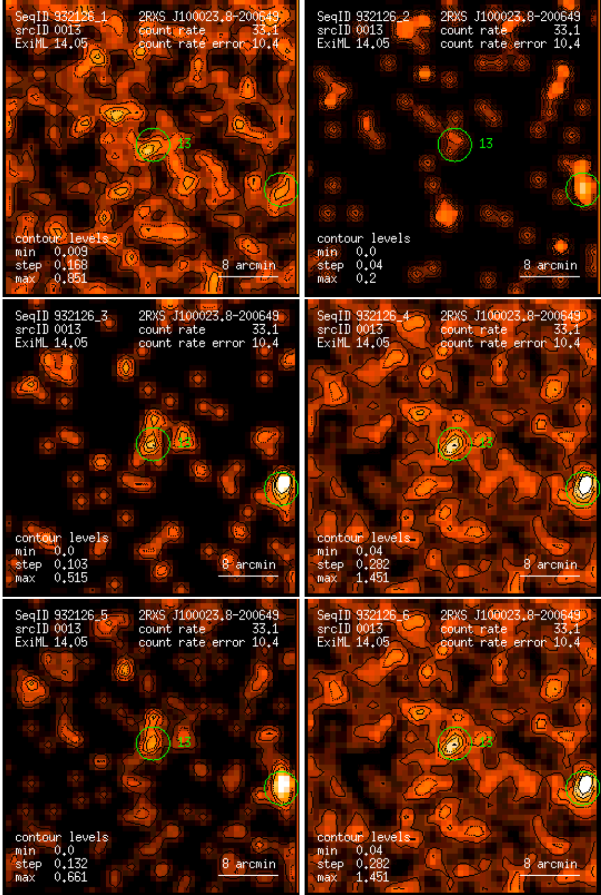
Figure 13: RASS 932126: detection 0013: band rate images, Gaussian filter: (1) PSPC channels 11 – 41, (2) 52 – 90, (3) 91 – 201, (4) 11 – 235, (5) 52 – 201, (6) 11 – 201. Broad band rates in counts/ks. Band rate contour levels in counts/ks/arcmin 2 .
