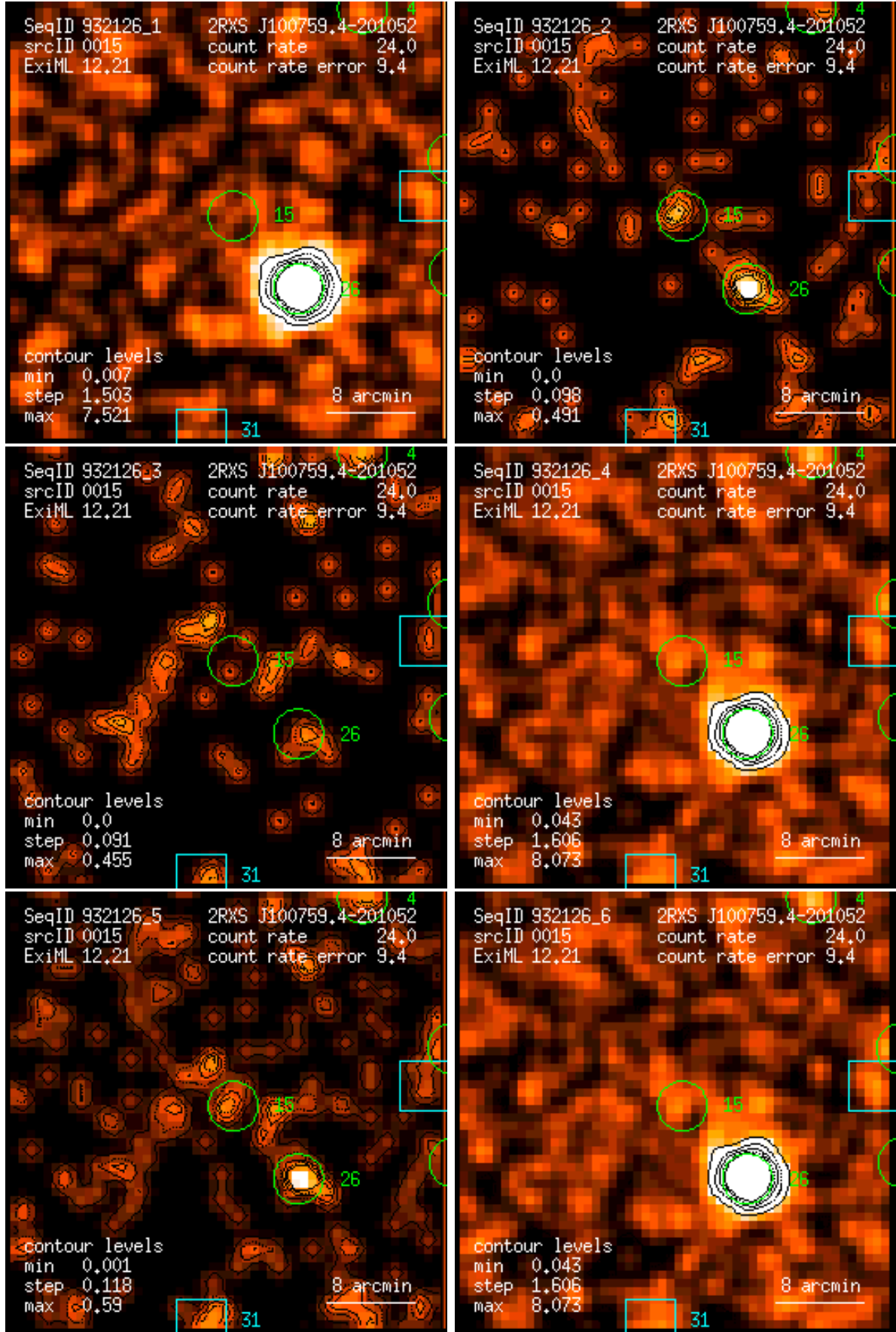
Figure 15: RASS 932126: detection 0015: band rate images, Gaussian filter: (1) PSPC channels 11 – 41, (2) 52 – 90, (3) 91 – 201, (4) 11 – 235, (5) 52 – 201, (6) 11 – 201. Broad band rates in counts/ks. Band rate contour levels in counts/ks/arcmin 2 .
