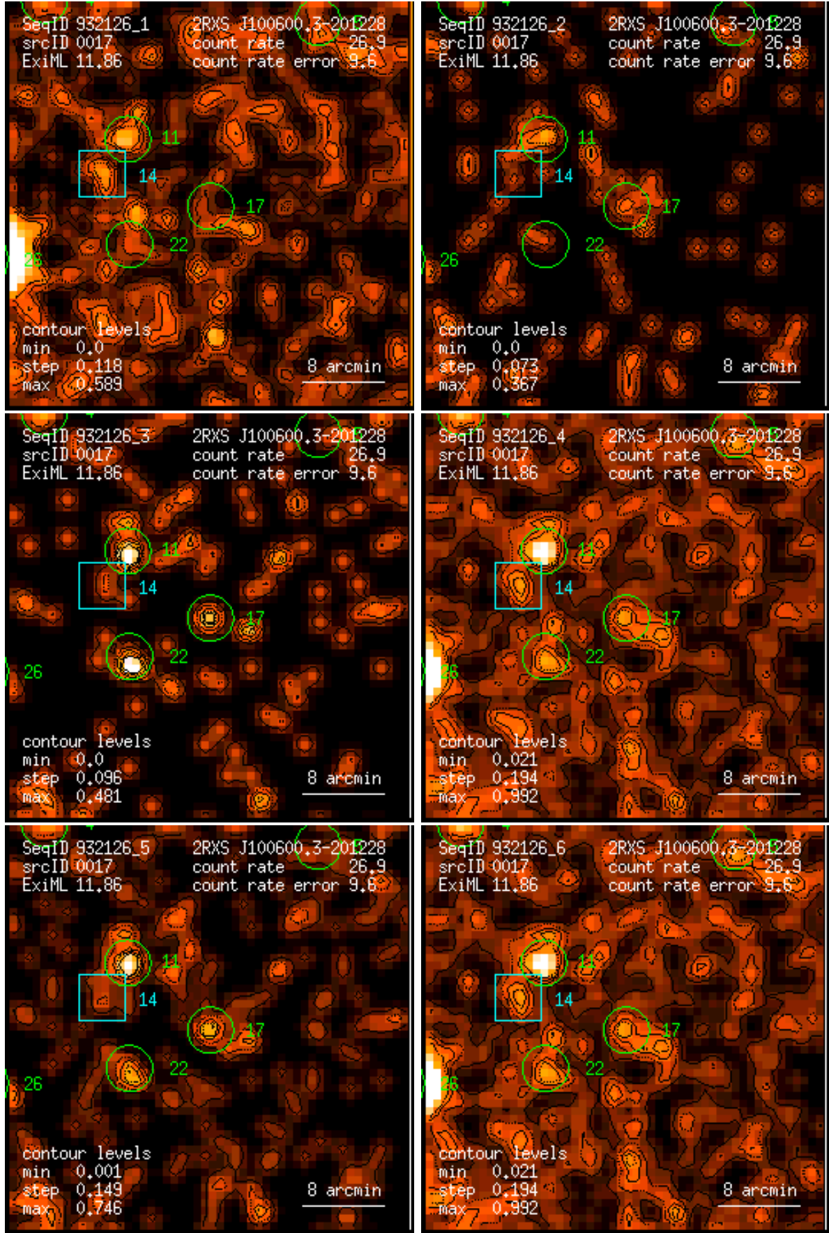
Figure 17: RASS 932126: detection 0017: band rate images, Gaussian filter: (1) PSPC channels 11 – 41, (2) 52 – 90, (3) 91 – 201, (4) 11 – 235, (5) 52 – 201, (6) 11 – 201. Broad band rates in counts/ks. Band rate contour levels in counts/ks/arcmin 2 .
