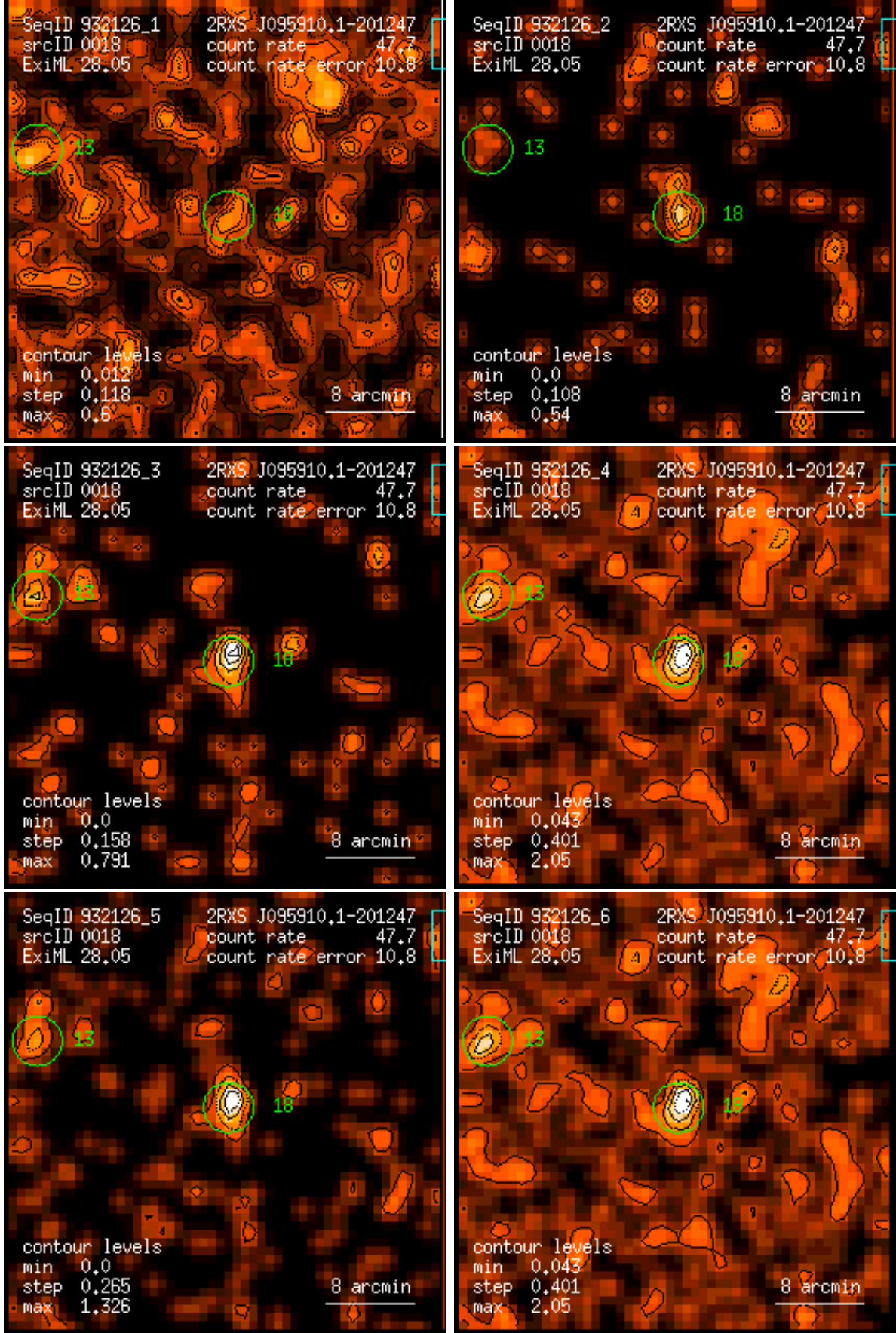
Figure 18: RASS 932126: detection 0018: band rate images, Gaussian filter: (1) PSPC channels 11 – 41, (2) 52 – 90, (3) 91 – 201, (4) 11 – 235, (5) 52 – 201, (6) 11 – 201. Broad band rates in counts/ks. Band rate contour levels in counts/ks/arcmin 2 .
