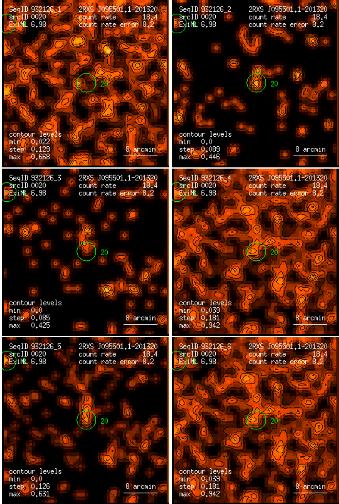
Figure 20: RASS 932126: detection 0020: band rate images, Gaussian filter: (1) PSPC channels 11 – 41, (2) 52 – 90, (3) 91 – 201, (4) 11 – 235, (5) 52 – 201, (6) 11 – 201. Broad band rates in counts/ks. Band rate contour levels in counts/ks/arcmin 2 .
