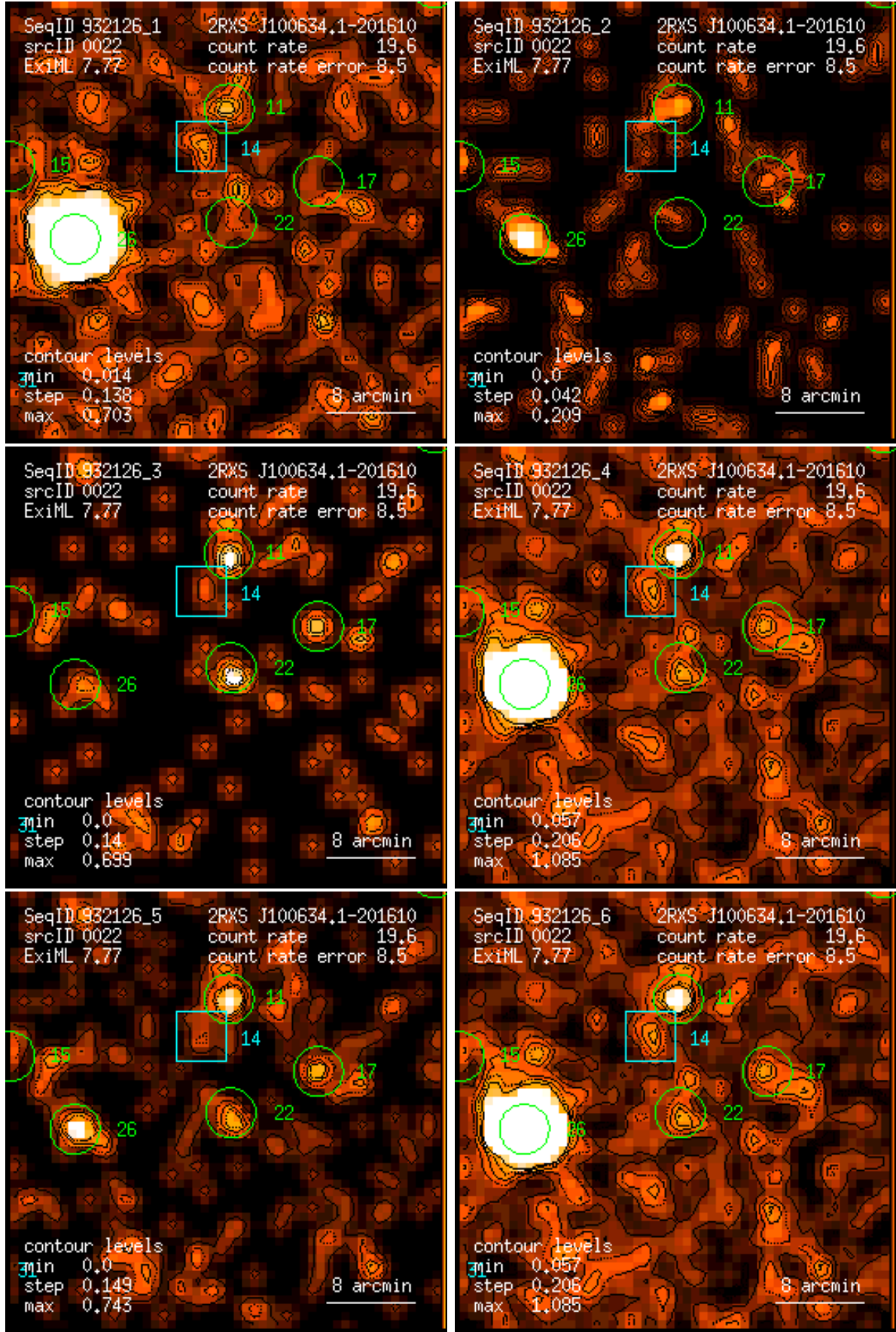
Figure 22: RASS 932126: detection 0022: band rate images, Gaussian filter: (1) PSPC channels 11 – 41, (2) 52 – 90, (3) 91 – 201, (4) 11 – 235, (5) 52 – 201, (6) 11 – 201. Broad band rates in counts/ks. Band rate contour levels in counts/ks/arcmin 2 .
