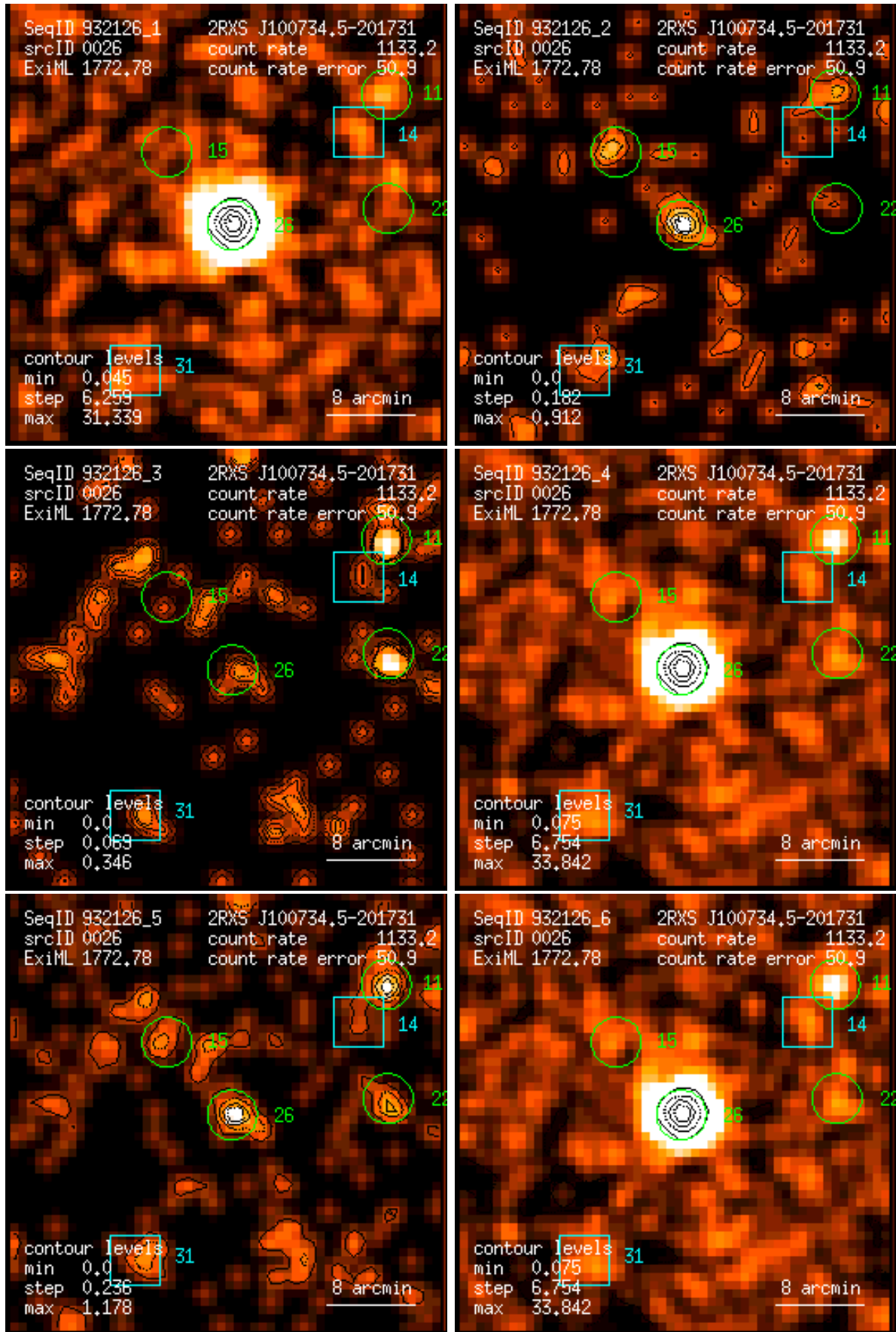
Figure 26: RASS 932126: detection 0026: band rate images, Gaussian filter: (1) PSPC channels 11 – 41, (2) 52 – 90, (3) 91 – 201, (4) 11 – 235, (5) 52 – 201, (6) 11 – 201. Broad band rates in counts/ks. Band rate contour levels in counts/ks/arcmin 2 .
