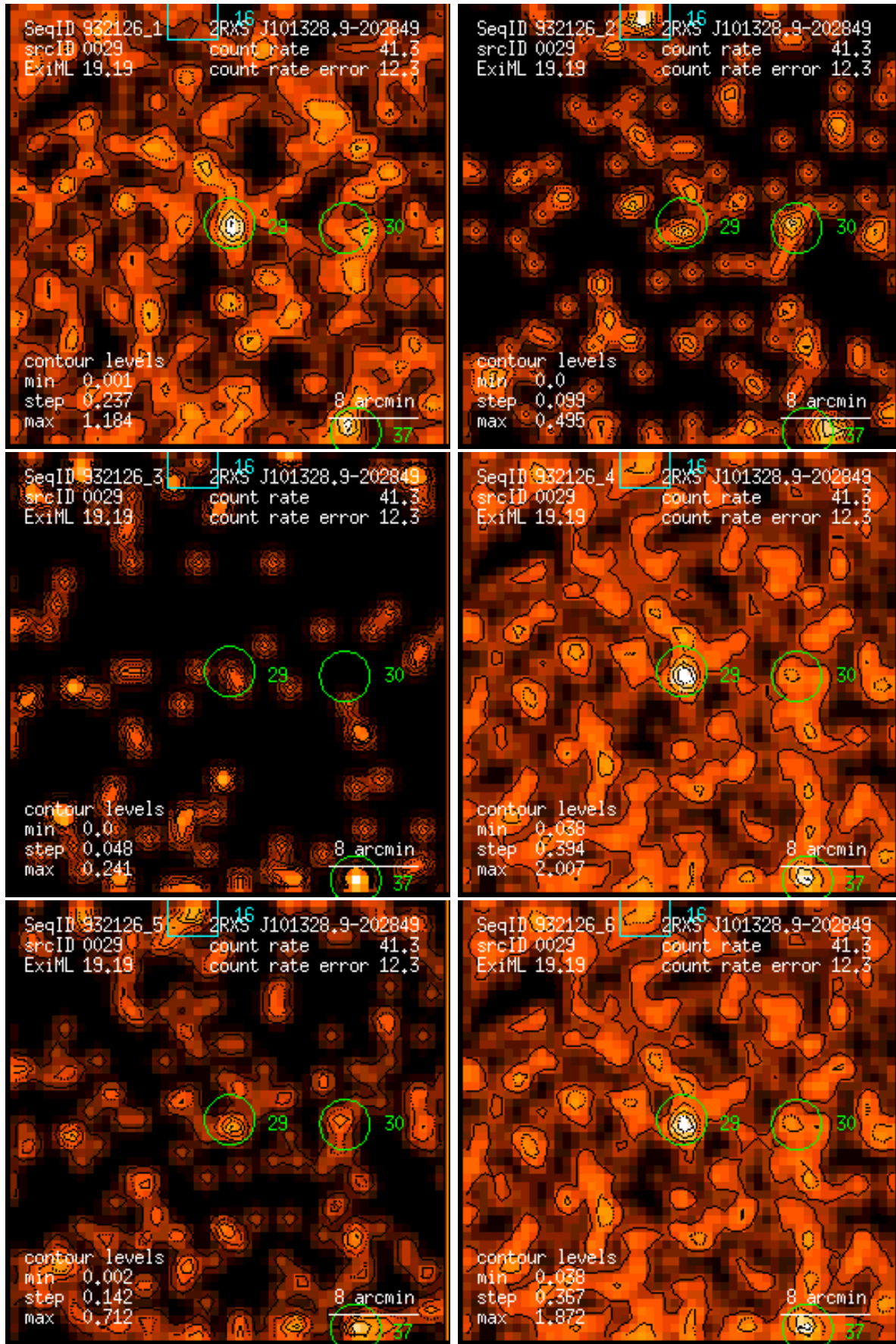
Figure 29: RASS 932126: detection 0029: band rate images, Gaussian filter: (1) PSPC channels 11 – 41, (2) 52 – 90, (3) 91 – 201, (4) 11 – 235, (5) 52 – 201, (6) 11 – 201. Broad band rates in counts/ks. Band rate contour levels in counts/ks/arcmin 2 .
