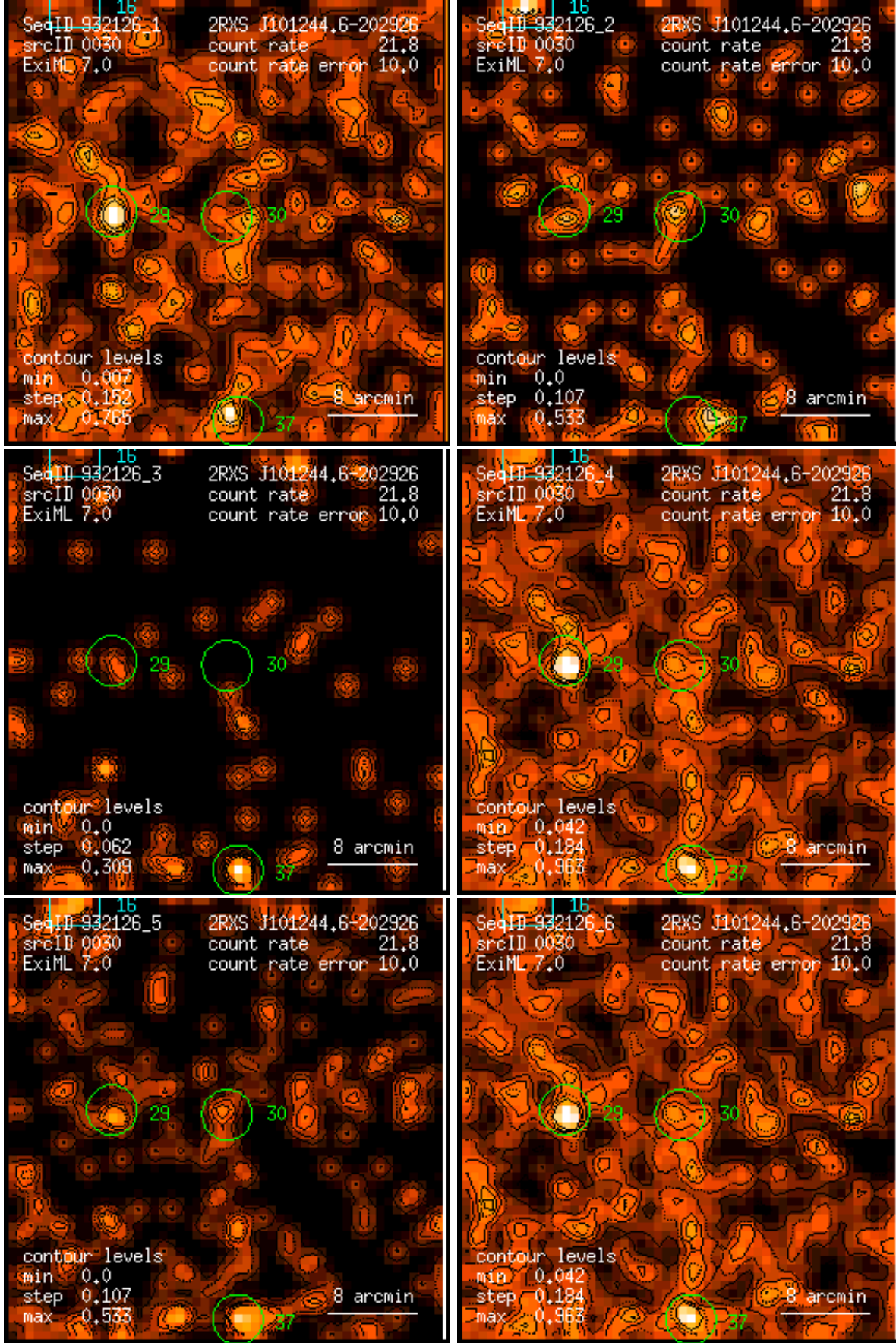
Figure 30: RASS 932126: detection 0030: band rate images, Gaussian filter: (1) PSPC channels 11 – 41, (2) 52 – 90, (3) 91 – 201, (4) 11 – 235, (5) 52 – 201, (6) 11 – 201. Broad band rates in counts/ks. Band rate contour levels in counts/ks/arcmin 2 .
