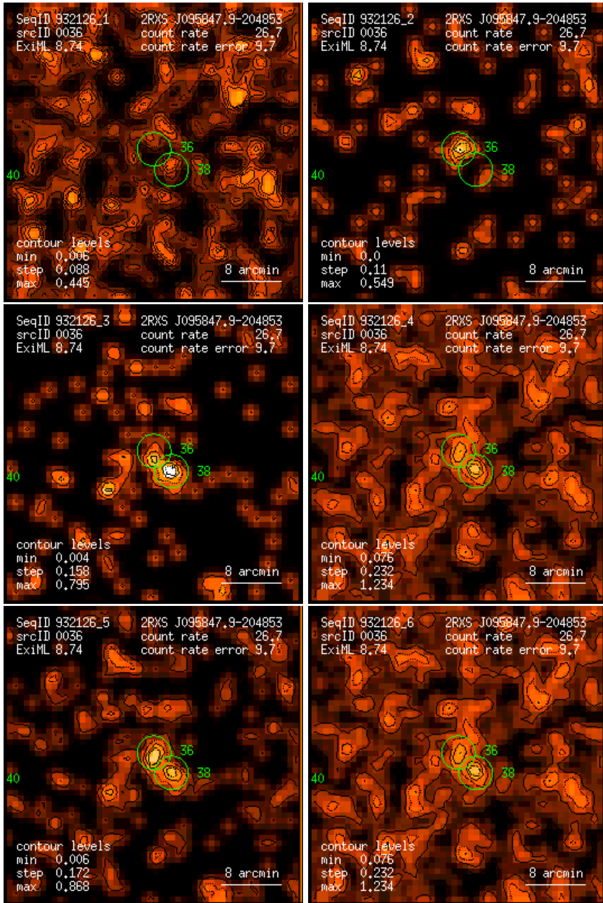
Figure 36: RASS 932126: detection 0036: band rate images, Gaussian filter: (1) PSPC channels 11 – 41, (2) 52 – 90, (3) 91 – 201, (4) 11 – 235, (5) 52 – 201, (6) 11 – 201. Broad band rates in counts/ks. Band rate contour levels in counts/ks/arcmin 2 .
