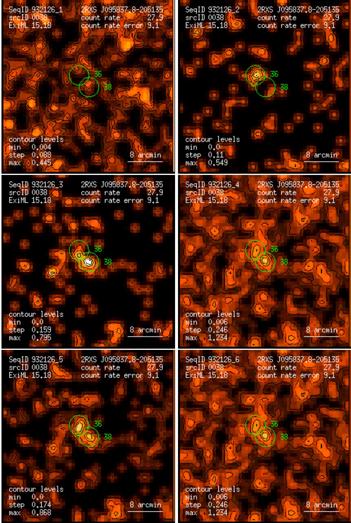
Figure 38: RASS 932126: detection 0038: band rate images, Gaussian filter: (1) PSPC channels 11 – 41, (2) 52 – 90, (3) 91 – 201, (4) 11 – 235, (5) 52 – 201, (6) 11 – 201. Broad band rates in counts/ks. Band rate contour levels in counts/ks/arcmin 2 .
