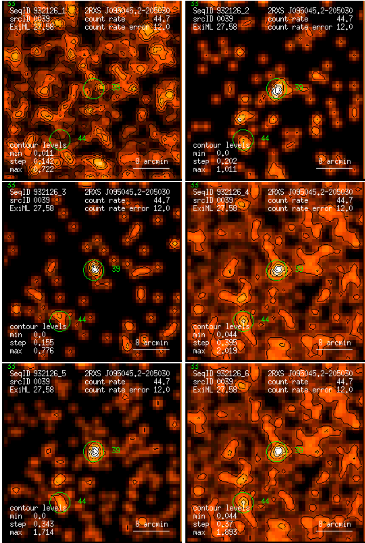
Figure 39: RASS 932126: detection 0039: band rate images, Gaussian filter: (1) PSPC channels 11 – 41, (2) 52 – 90, (3) 91 – 201, (4) 11 – 235, (5) 52 – 201, (6) 11 – 201. Broad band rates in counts/ks. Band rate contour levels in counts/ks/arcmin 2 .
