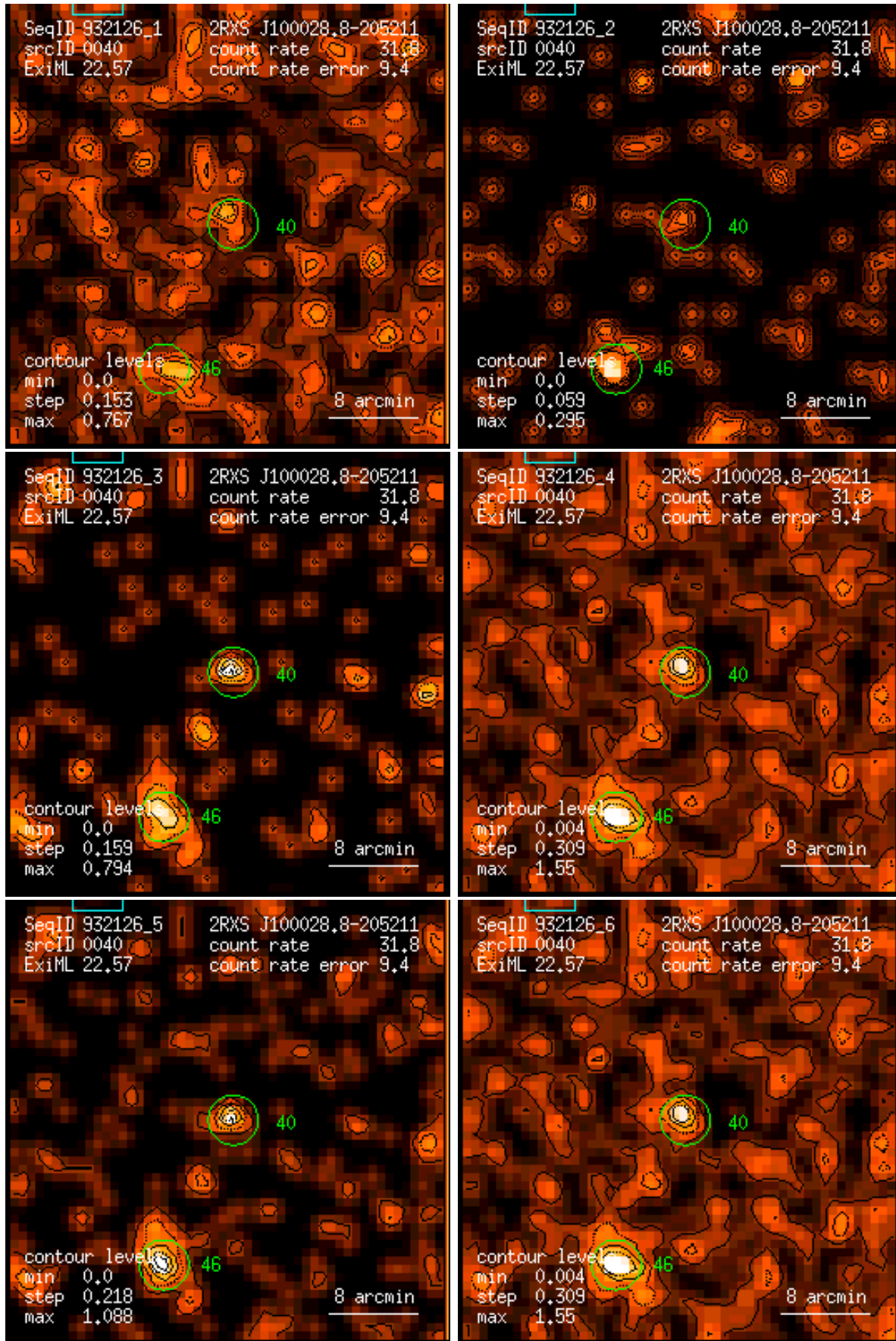
Figure 40: RASS 932126: detection 0040: band rate images, Gaussian filter: (1) PSPC channels 11 – 41, (2) 52 – 90, (3) 91 – 201, (4) 11 – 235, (5) 52 – 201, (6) 11 – 201. Broad band rates in counts/ks. Band rate contour levels in counts/ks/arcmin 2 .
