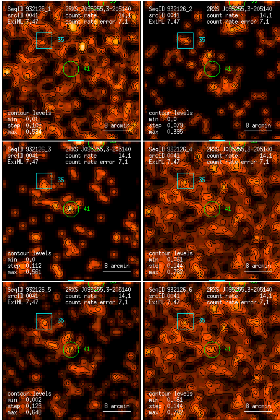
Figure 41: RASS 932126: detection 0041: band rate images, Gaussian filter: (1) PSPPC channels 11 – 41, (2) 52 – 90, (3) 91 – 201, (4) 11 – 235, (5) 52 – 201, (6) 11 – 201. Broad band rates in counts/ks. Band rate contour levels in counts/ks/arcmin 2 .
