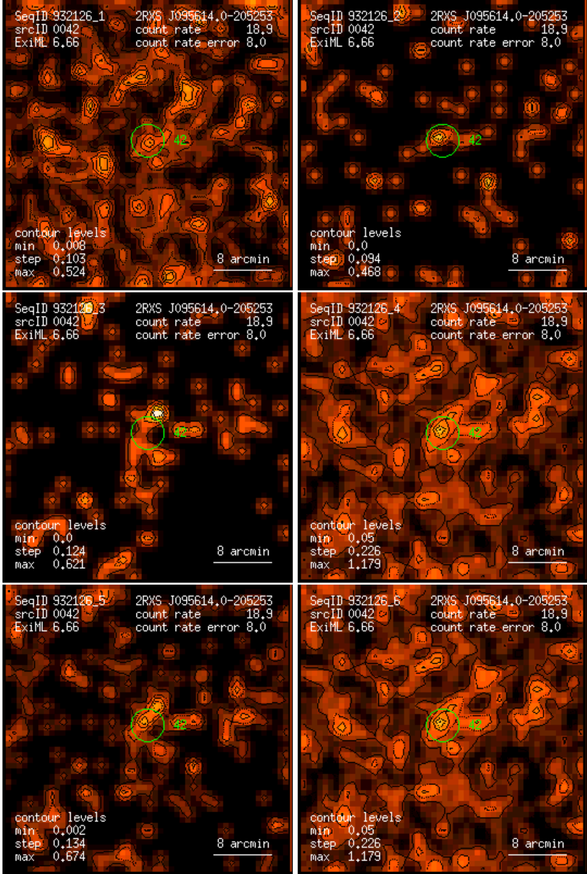
Figure 42: RASS 932126: detection 0042: band rate images, Gaussian filter: (1) PSPC channels 11 – 41, (2) 52 – 90, (3) 91 – 201, (4) 11 – 235, (5) 52 – 201, (6) 11 – 201. Broad band rates in counts/ks. Band rate contour levels in counts/ks/arcmin 2 .
