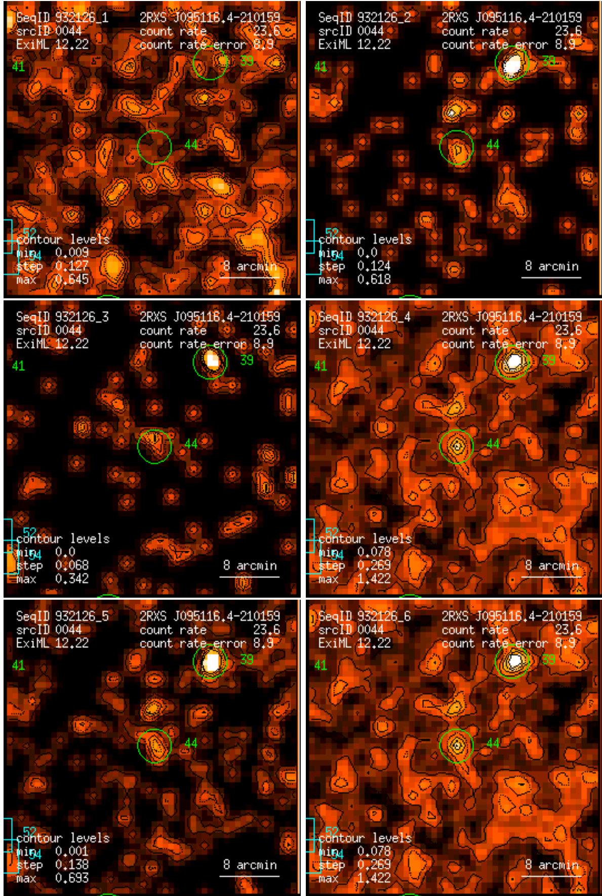
Figure 44: RASS 932126: detection 0044: band rate images, Gaussian filter: (1) PSPPC channels 11 – 41, (2) 52 – 90, (3) 91 – 201, (4) 11 – 235, (5) 52 – 201, (6) 11 – 201. Broad band rates in counts/ks. Band rate contour levels in counts/ks/arcmin 2 .
