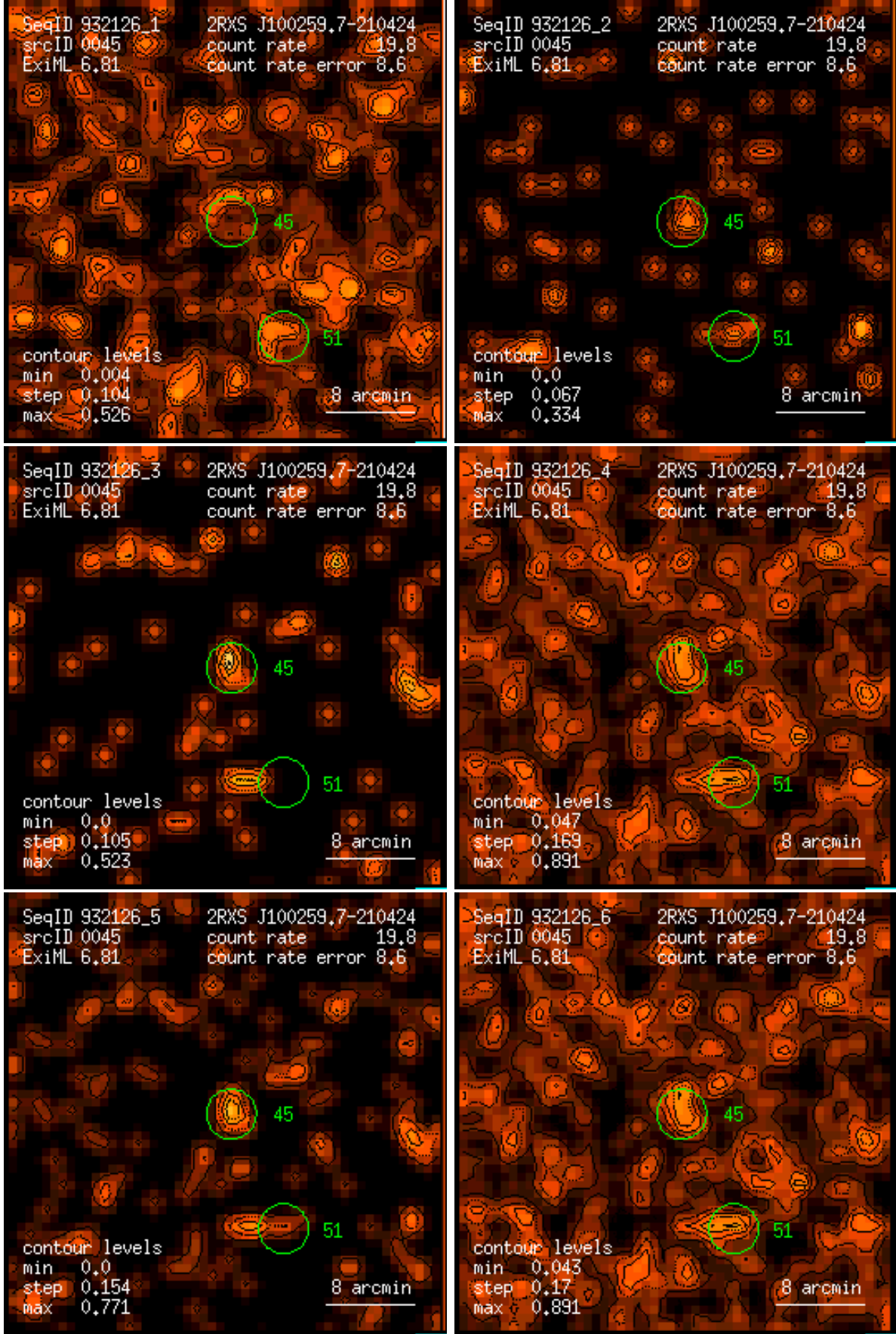
Figure 45: RASS 932126: detection 0045: band rate images, Gaussian filter: (1) PSPC channels 11 – 41, (2) 52 – 90, (3) 91 – 201, (4) 11 – 235, (5) 52 – 201, (6) 11 – 201. Broad band rates in counts/ks. Band rate contour levels in counts/ks/arcmin 2 .
