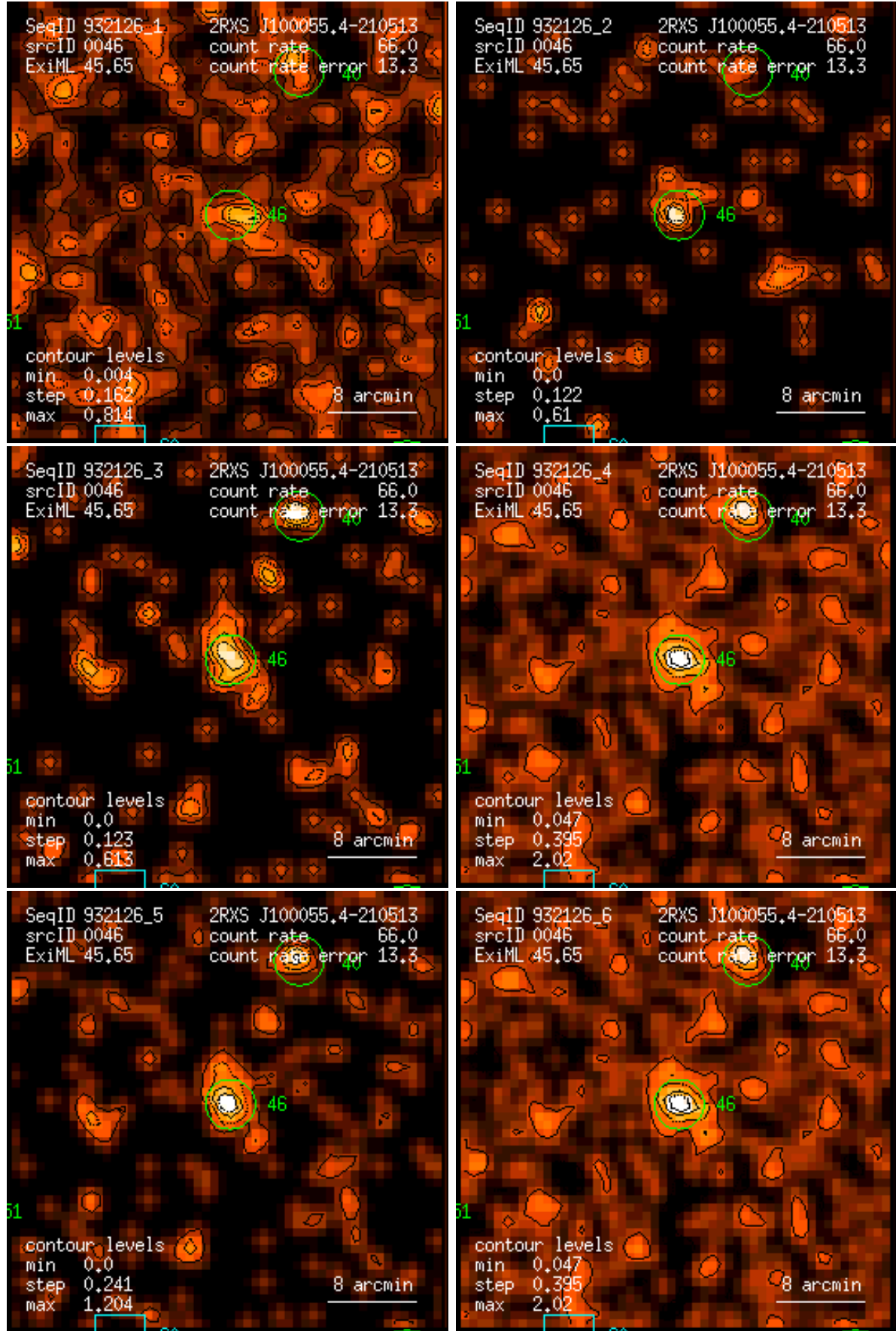
Figure 46: RASS 932126: detection 0046: band rate images, Gaussian filter: (1) PSPC channels 11 – 41, (2) 52 – 90, (3) 91 – 201, (4) 11 – 235, (5) 52 – 201, (6) 11 – 201. Broad band rates in counts/ks. Band rate contour levels in counts/ks/arcmin 2 .
