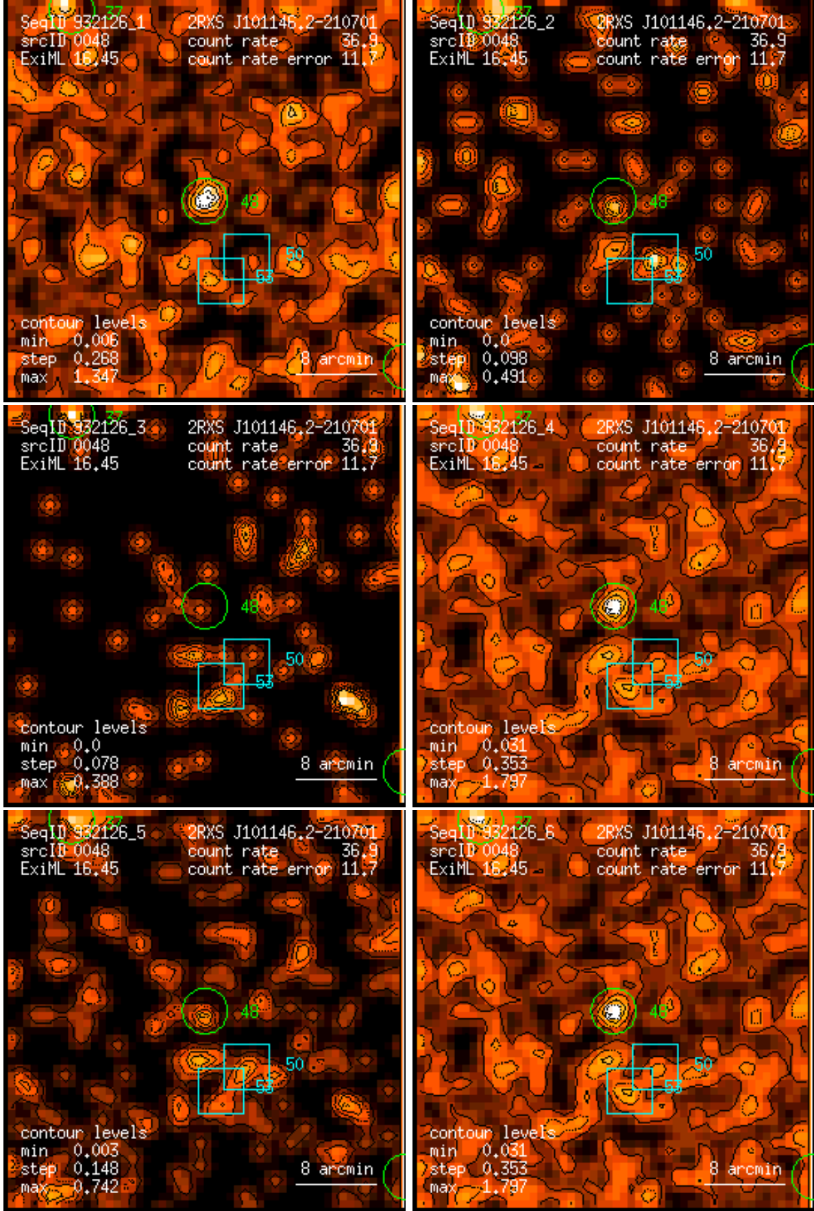
Figure 48: RASS 932126: detection 0048: band rate images, Gaussian filter: (1) PSPC channels 11 – 41, (2) 52 – 90, (3) 91 – 201, (4) 11 – 235, (5) 52 – 201, (6) 11 – 201. Broad band rates in counts/ks. Band rate contour levels in counts/ks/arcmin 2 .
