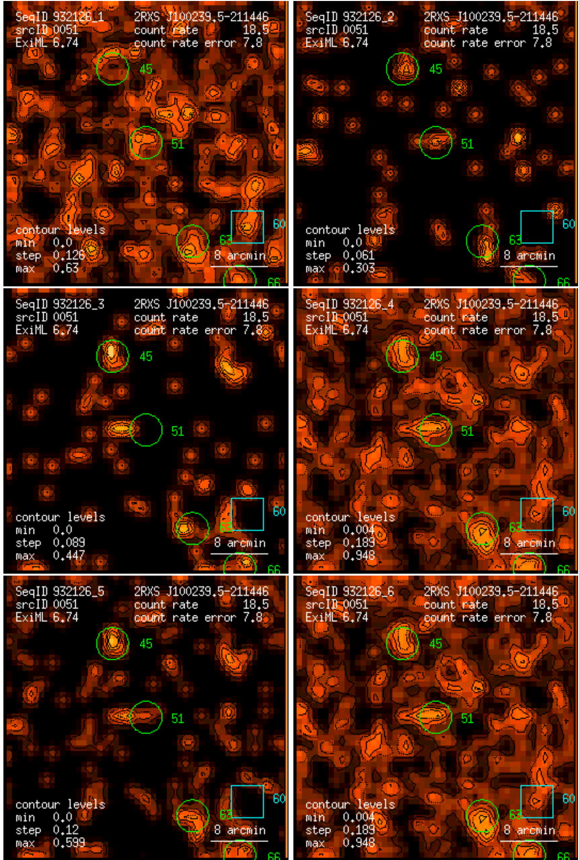
Figure 51: RASS 932126: detection 0051: band rate images, Gaussian filter: (1) PSPPC channels 11 – 41, (2) 52 – 90, (3) 91 – 201, (4) 11 – 235, (5) 52 – 201, (6) 11 – 201. Broad band rates in counts/ks. Band rate contour levels in counts/ks/arcmin 2 .
