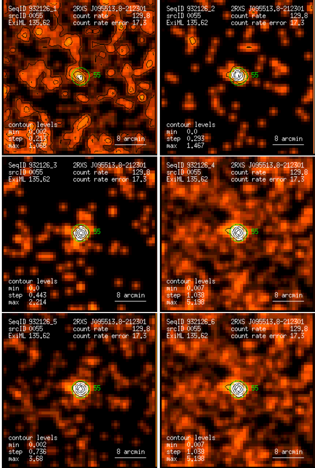
Figure 55: RASS 932126: detection 0055: band rate images, Gaussian filter: (1) PSPC channels 11 – 41, (2) 52 – 90, (3) 91 – 201, (4) 11 – 235, (5) 52 – 201, (6) 11 – 201. Broad band rates in counts/ks. Band rate contour levels in counts/ks/arcmin 2 .
