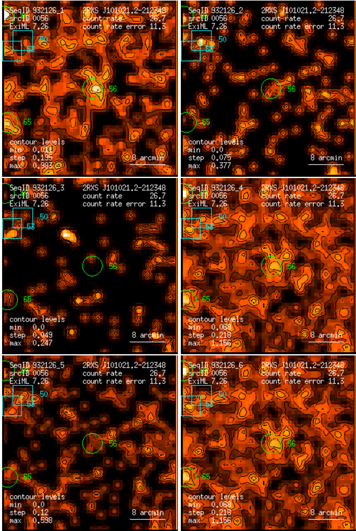
Figure 56: RASS 932126: detection 0056: band rate images, Gaussian filter: (1) PSPC channels 11 – 41, (2) 52 – 90, (3) 91 – 201, (4) 11 – 235, (5) 52 – 201, (6) 11 – 201. Broad band rates in counts/ks. Band rate contour levels in counts/ks/arcmin 2 .
