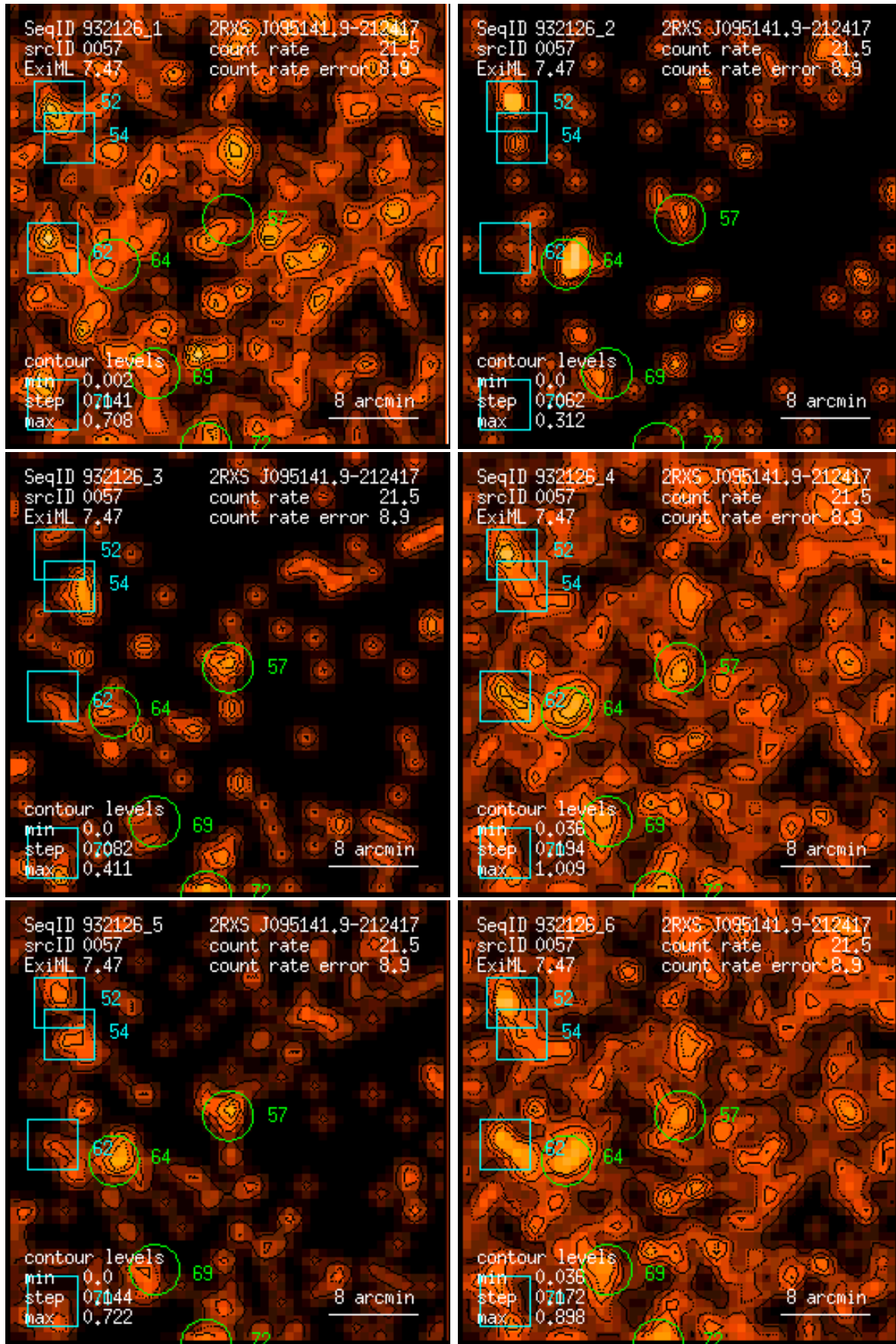
Figure 57: RASS 932126: detection 0057: band rate images, Gaussian filter: (1) PSPC channels 11 – 41, (2) 52 – 90, (3) 91 – 201, (4) 11 – 235, (5) 52 – 201, (6) 11 – 201. Broad band rates in counts/ks. Band rate contour levels in counts/ks/arcmin 2 .
