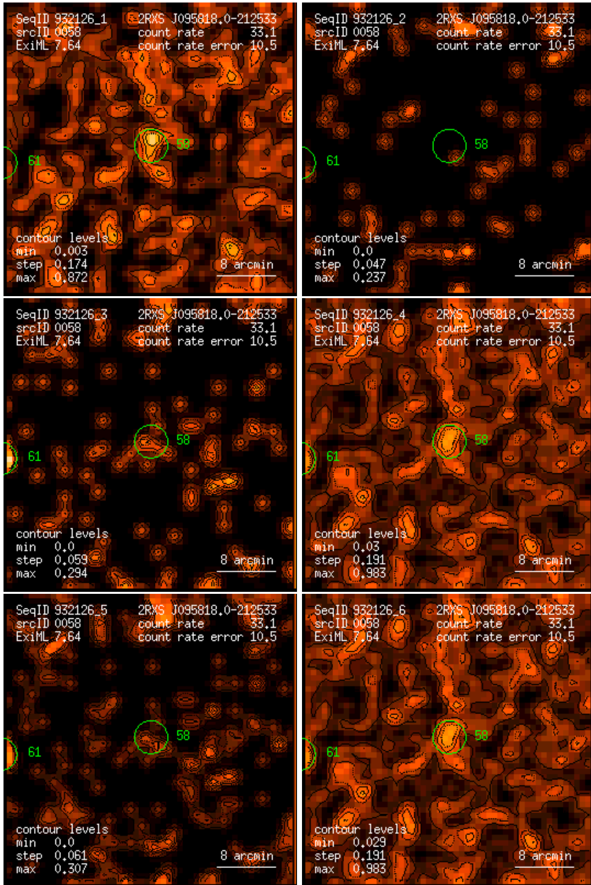
Figure 58: RASS 932126: detection 0058: band rate images, Gaussian filter: (1) PSPP channels 11 – 41, (2) 52 – 90, (3) 91 – 201, (4) 11 – 235, (5) 52 – 201, (6) 11 – 201. Broad band rates in counts/ks. Band rate contour levels in counts/ks/arcmin 2 .
